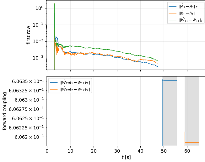
Figure 2. The first stage under the noise (43). Top: running batch estimates, matrices in the Frobenius norm, vectors in the Euclidean norm, of the three blocks of the first row over the regression window [r_1 + T, r'_1] = [3, 47.5] . Bottom: the forward coupling W_{12} , recovered column by column on the two saturation windows (shaded): during window i \in \{1, 2\} the steering law holds S(V_2) = e_i on [t_i, t_i + \tau + T] , so the residual (13e) equals W_{12}e_i , and each column estimate is the running average of \phi_1 e_i^T over [t_i + T, t_i + \tau + T] .
