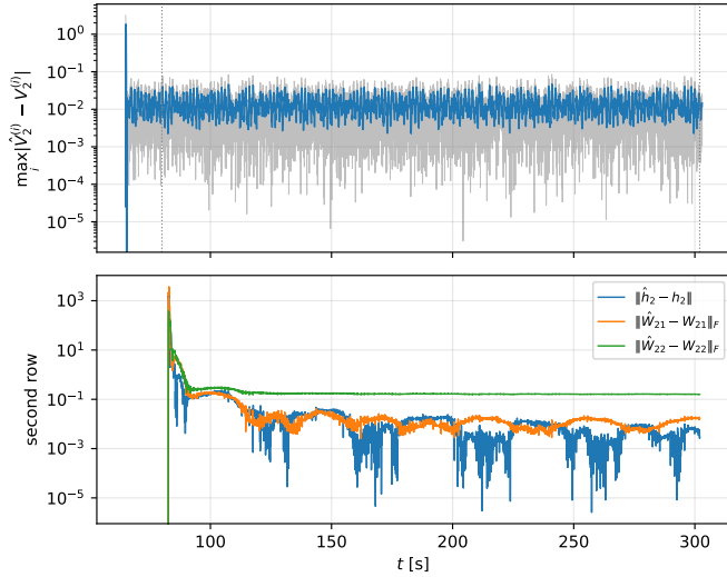
Figure 3. The second stage under the noise (43). Top: reconstruction error \max_i |\hat{V}_2^{(i)} - V_2^{(i)}| from the descent on, raw trace light and envelope solid, on a logarithmic scale. The envelope is the raw trace passed through a low-pass (second-order Butterworth, cutoff 3 rad/s) and is shown for readability only. Dotted lines mark the end of the descent (time 80) and the delivery r'_2 = 302 . Bottom: the three blocks of the second row over [r_2 + T, r'_2] = [82.5, 302] , computed on causally filtered signals with cutoff 5 rad/s.
