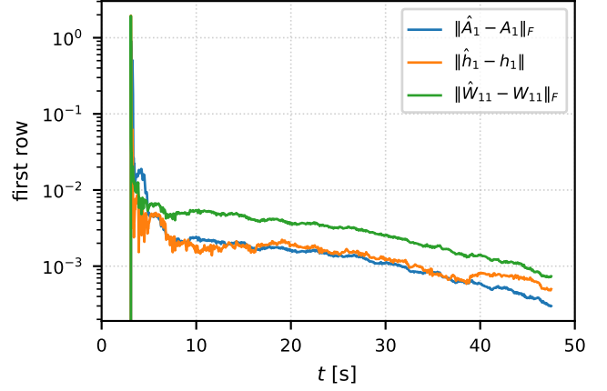
Figure 2. The first stage under the noise (43): running batch estimates, matrices in the Frobenius norm, vectors in the Euclidean norm, of the three blocks of the first row over the regression window [r_1 + T, r'_1] = [3, 47.5] .
