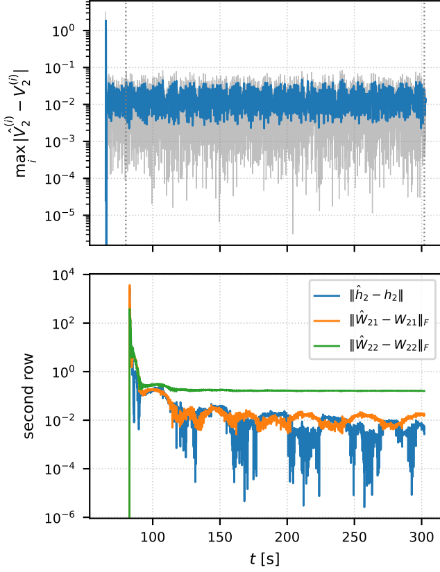
Figure 3. The second stage under the noise (43). Top: reconstruction error \max_i |\hat{V}_2^{(i)} - V_2^{(i)}| from the descent on, raw trace light and envelope solid, on a logarithmic scale. The envelope is the raw trace passed through a low-pass (second-order Butterworth, cutoff 3 rad/s) and is shown for readability only. Dotted lines mark the end of the descent (time 80) and the delivery r'_2 = 302 . Bottom: the three blocks of the second row over [r_2 + T, r'_2] = [82.5, 302] , computed on causally filtered signals with cutoff 5 rad/s.
