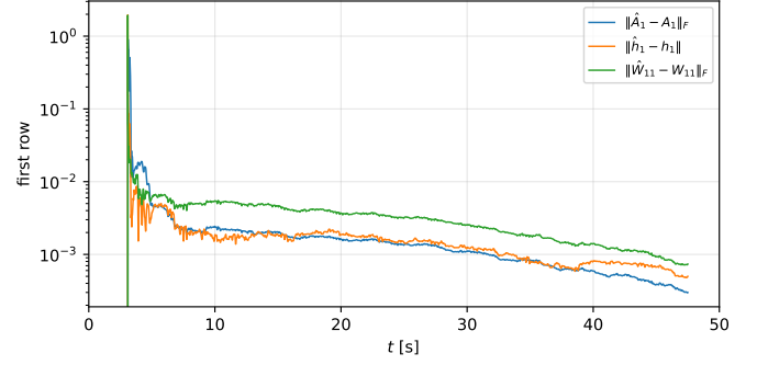
Figure 2. The first stage under the noise (43): running batch estimates, matrices in the Frobenius norm, vectors in the Euclidean norm, of the three blocks of the first row over the regression window [r_1 + T, r'_1] = [3, 47.5] .
