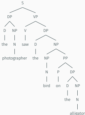
Bird-on-alligator tree
