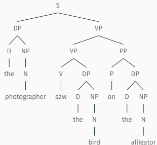
Photographer-on-alligator tree
