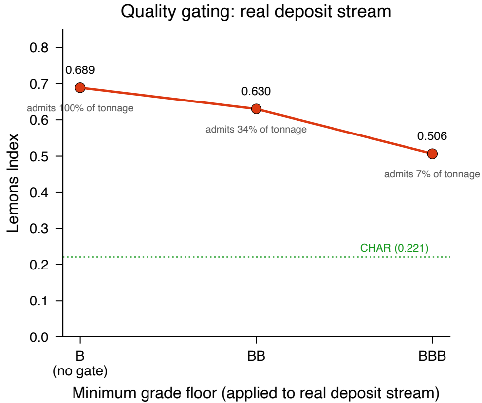
Fig. 4 Illustrative quality gates applied retrospectively to the observed BCT deposit stream. A gate admits credits at or above an author-defined grade threshold: B admits all credits, whereas BB and BBB impose progressively higher thresholds. The deposit-tonnage-weighted Pool Quality Deficit (PQD, also called the Lemons Index) is lower for higher assessed quality; the other axis is the share of observed tonnage that would be admitted. A BBB threshold lowers PQD from 0.689 to 0.506 but would admit 7.2% of tonnage. CHAR is a separate pool restricted to an allowlist of credit categories; its PQD is 0.221. These are mechanical counterfactuals, not estimates of market behaviour after a gate is introduced.
