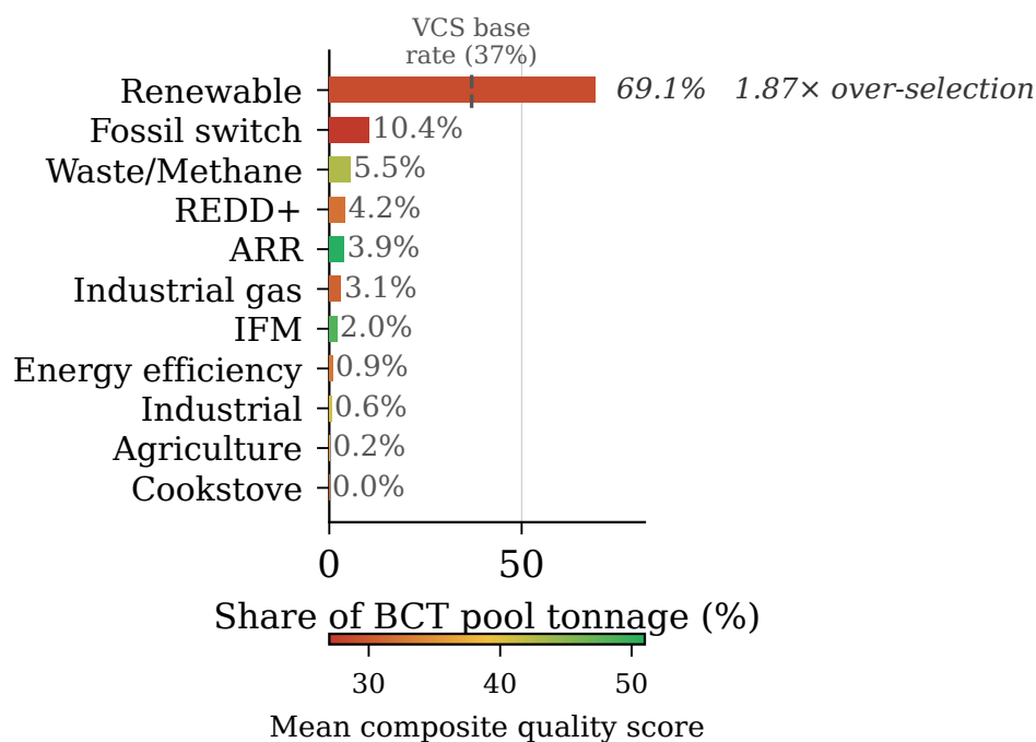
Fig. 1 Composition of the Base Carbon Tonne (BCT) pool by credit methodology. Bars show each category's share of the approximately 22 million tCO 2 represented by all 1,187 on-chain deposits; shares are weighted by deposited tonnage, not by projects or transactions. Renewable-energy credits account for 69.1% of deposited tonnage, whereas REDD+ (credits intended to reduce emissions from deforestation and forest degradation) accounts for 4.2%.
