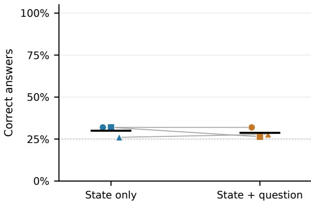
b Paired test accuracy
