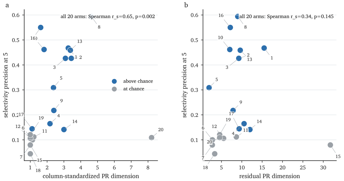
Figure S3: Exploratory DTI association on the complete 20-arm panel. Selectivity precision at five is plotted against the column-standardized PR effective dimension ( a ) and the two-way-centered residual PR effective dimension ( b ). Numbers identify arms in Table S5; blue denotes arms above the outcome-related chance criterion and grey denotes arms at chance. Correlations are descriptive because the arms share data, architectures and representations.
