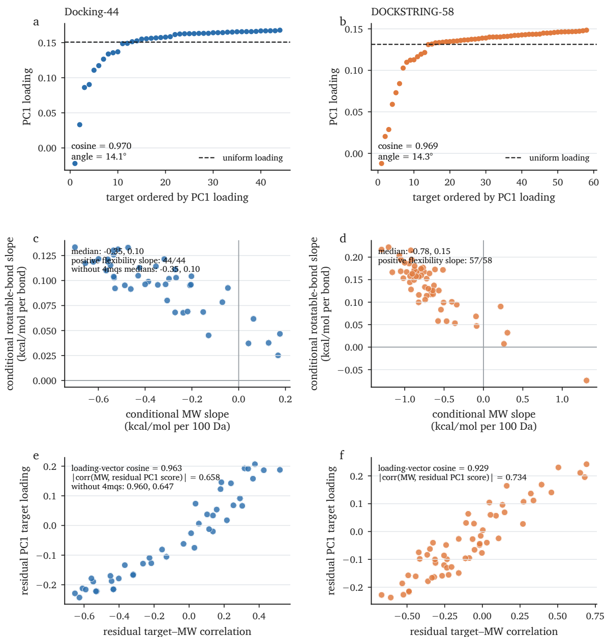
Figure S5: Shared-axis loadings are uniform; residual loadings track target-specific size dependence. a,b, Sorted raw PC1 target loadings and the uniform-loading reference. c,d, Conditional molecular-weight and RDKit rotatable-bond slopes for each target. e,f, Alignment of target-wise residual molecular-weight correlations with residual PC1 target loadings. Component signs are oriented by the molecular-weight vector and have no intrinsic meaning.
