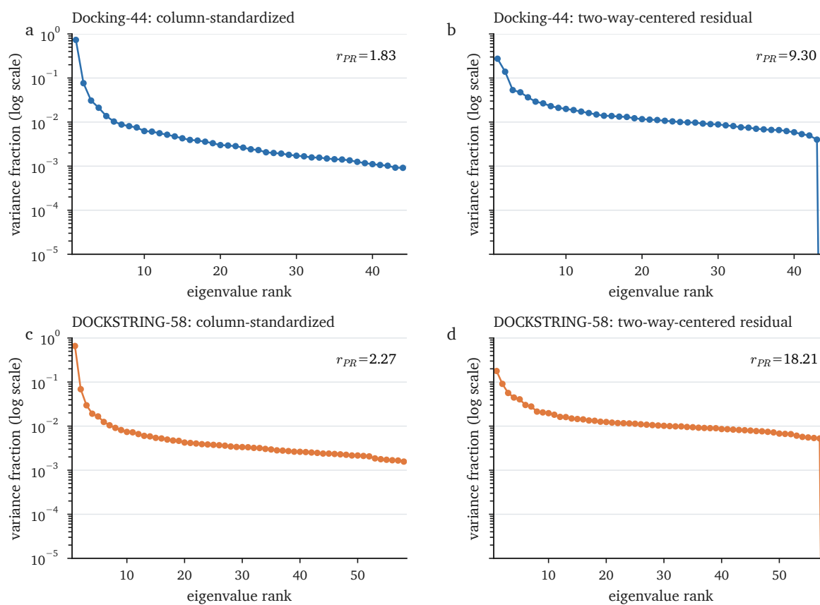
Figure S1: Full correlation-spectrum scree plots. a,b, Docking-44 column-standardized and two-way-residual spectra. c,d, DOCKSTRING-58 column-standardized and two-way-residual spectra. Eigenvalues are divided by the number of targets so each spectrum sums to one. The ordinate is logarithmic. Two-way centring imposes one exact zero residual eigenvalue.
