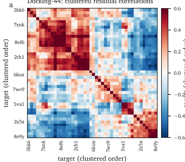
Docking-44: clustered residual correlations
