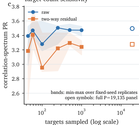
Target-count sensitivity
