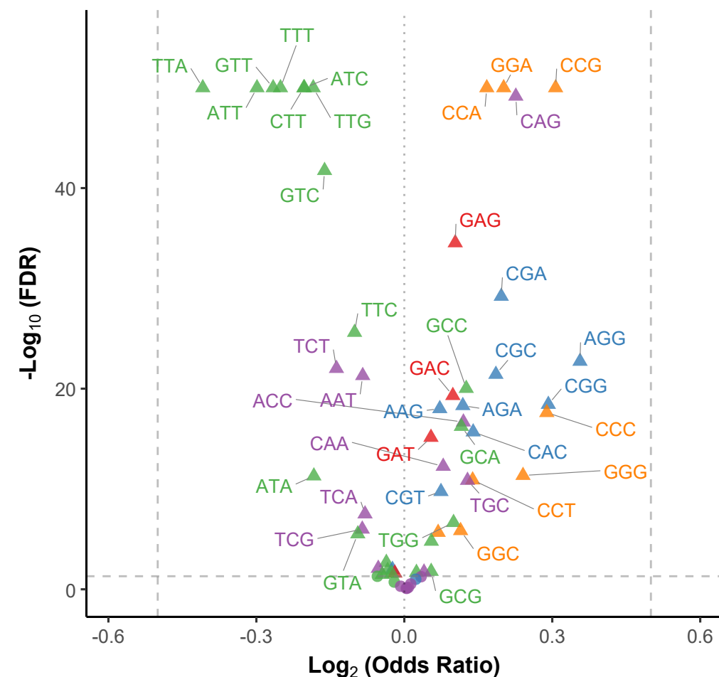
P-site | control
