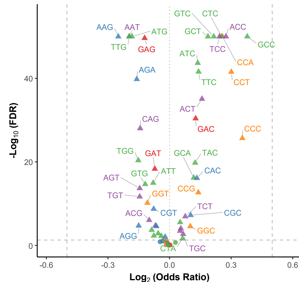
E-site | control
