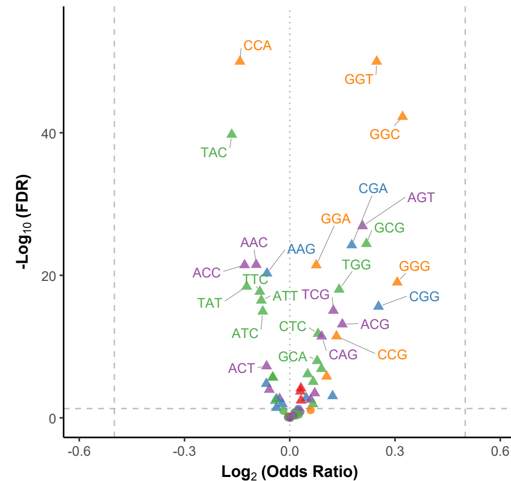
E-site | BWM
