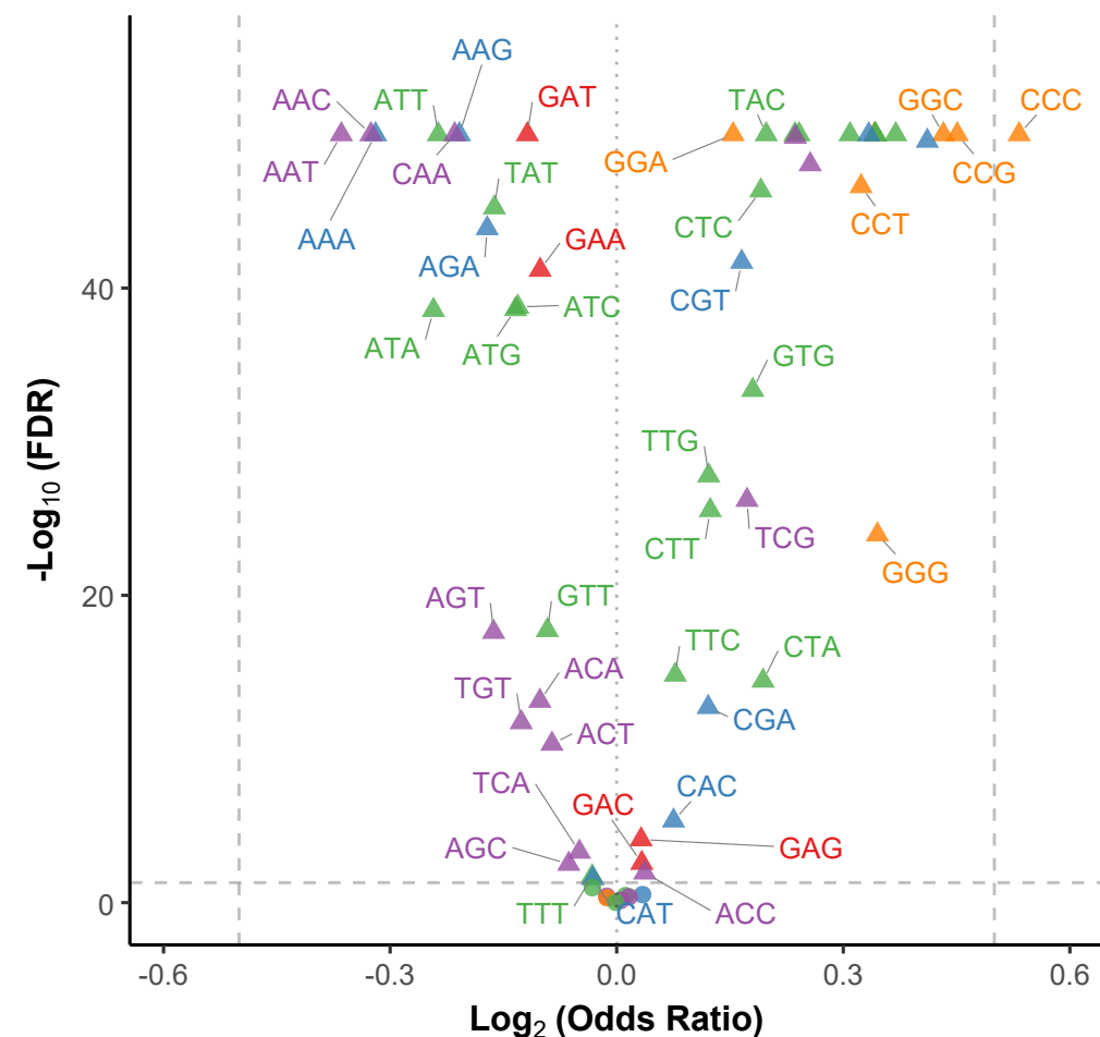
A-site | control
