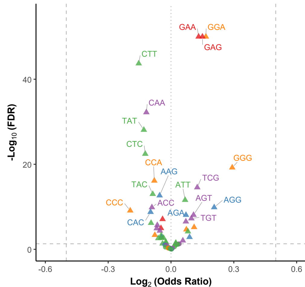
A-site | BWM
