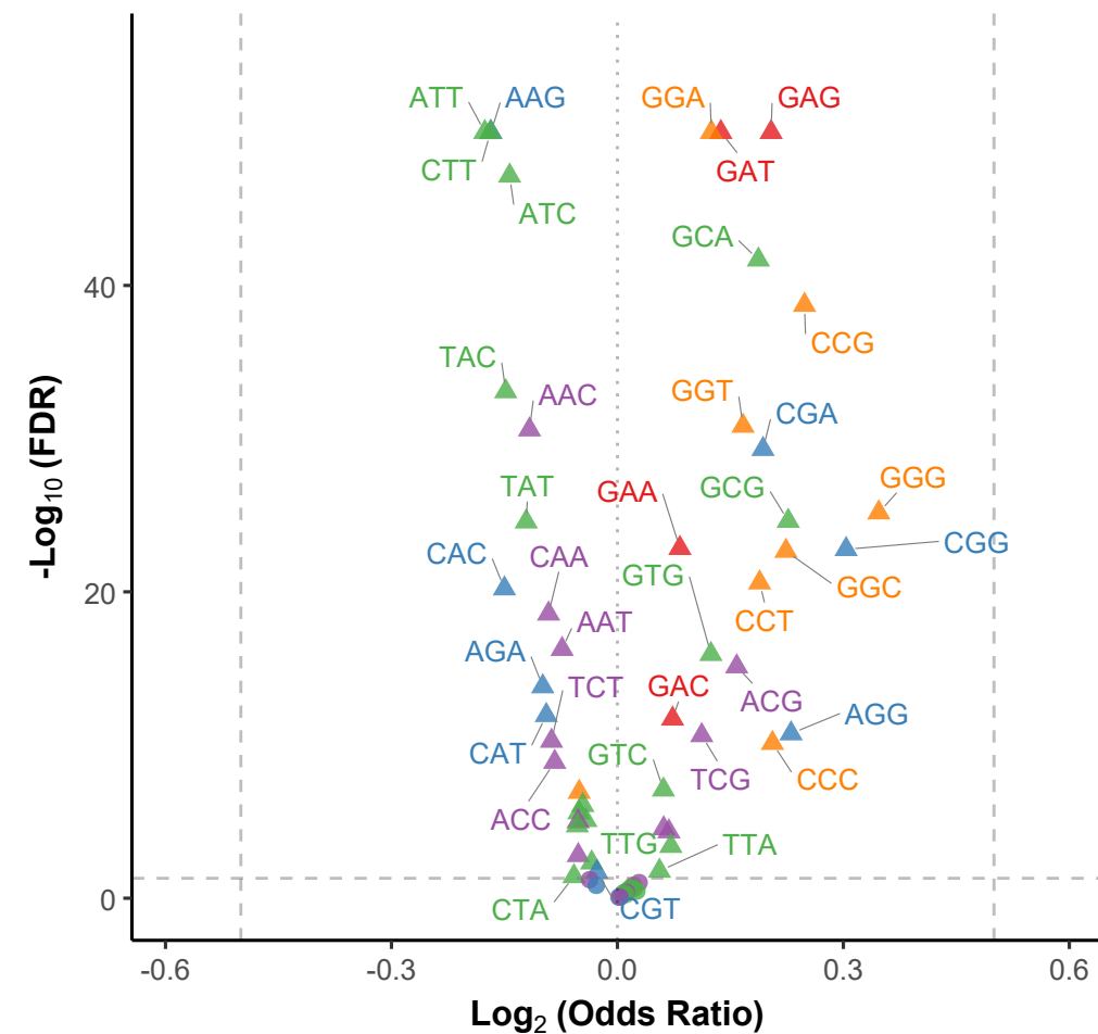
P-site | BWM
