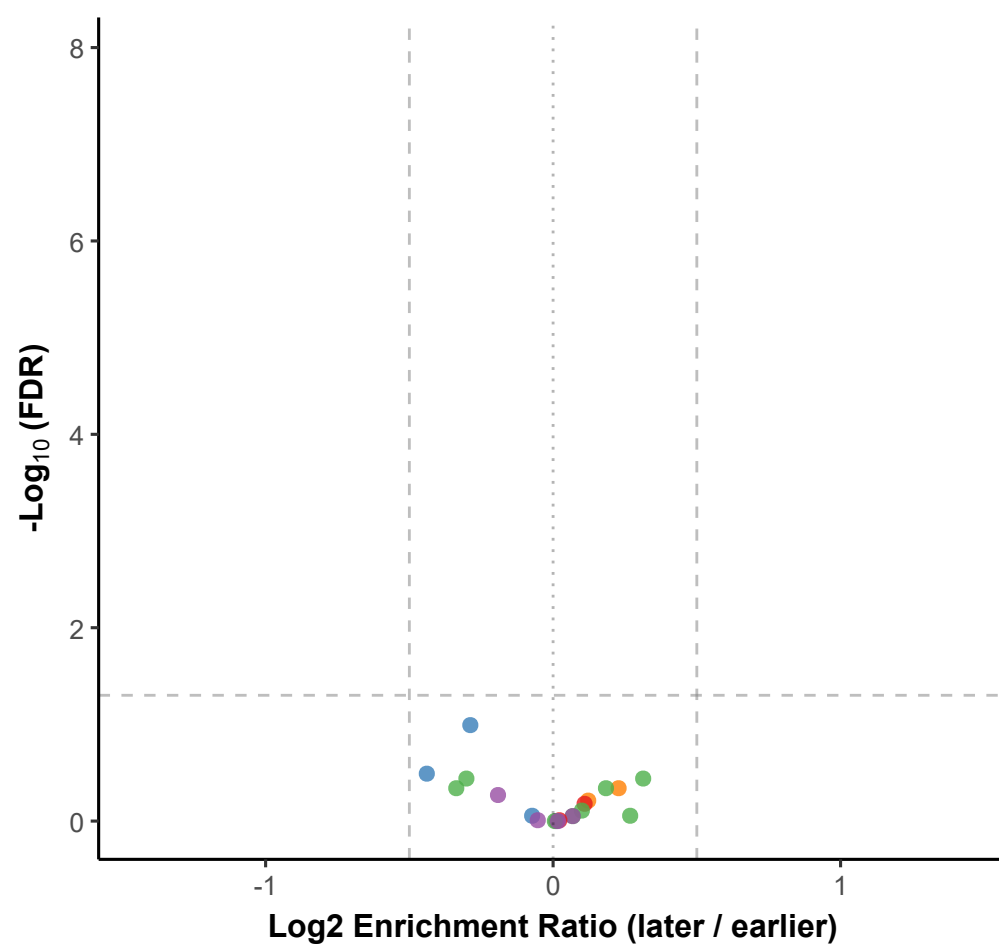
P-site | d5 vs d0
