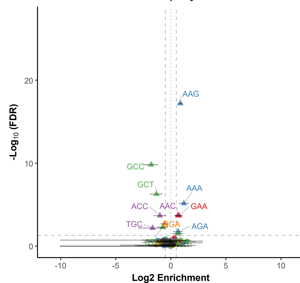
E-site | Day 5
