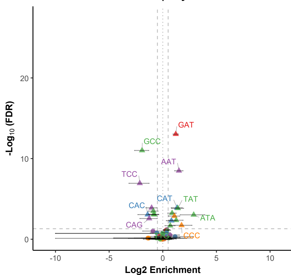
P-site | Day 5
