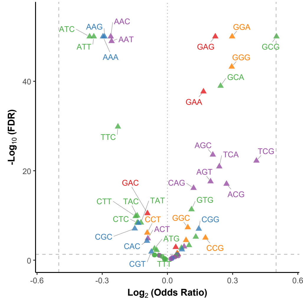
P-site
