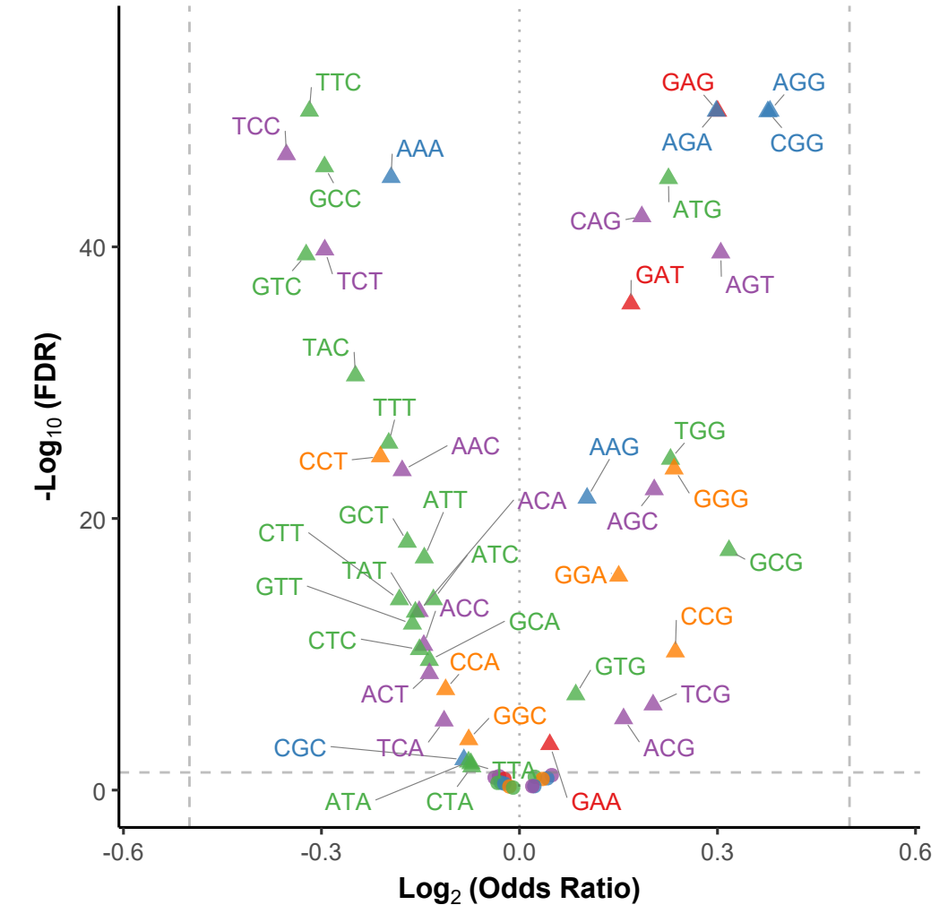
E-site
