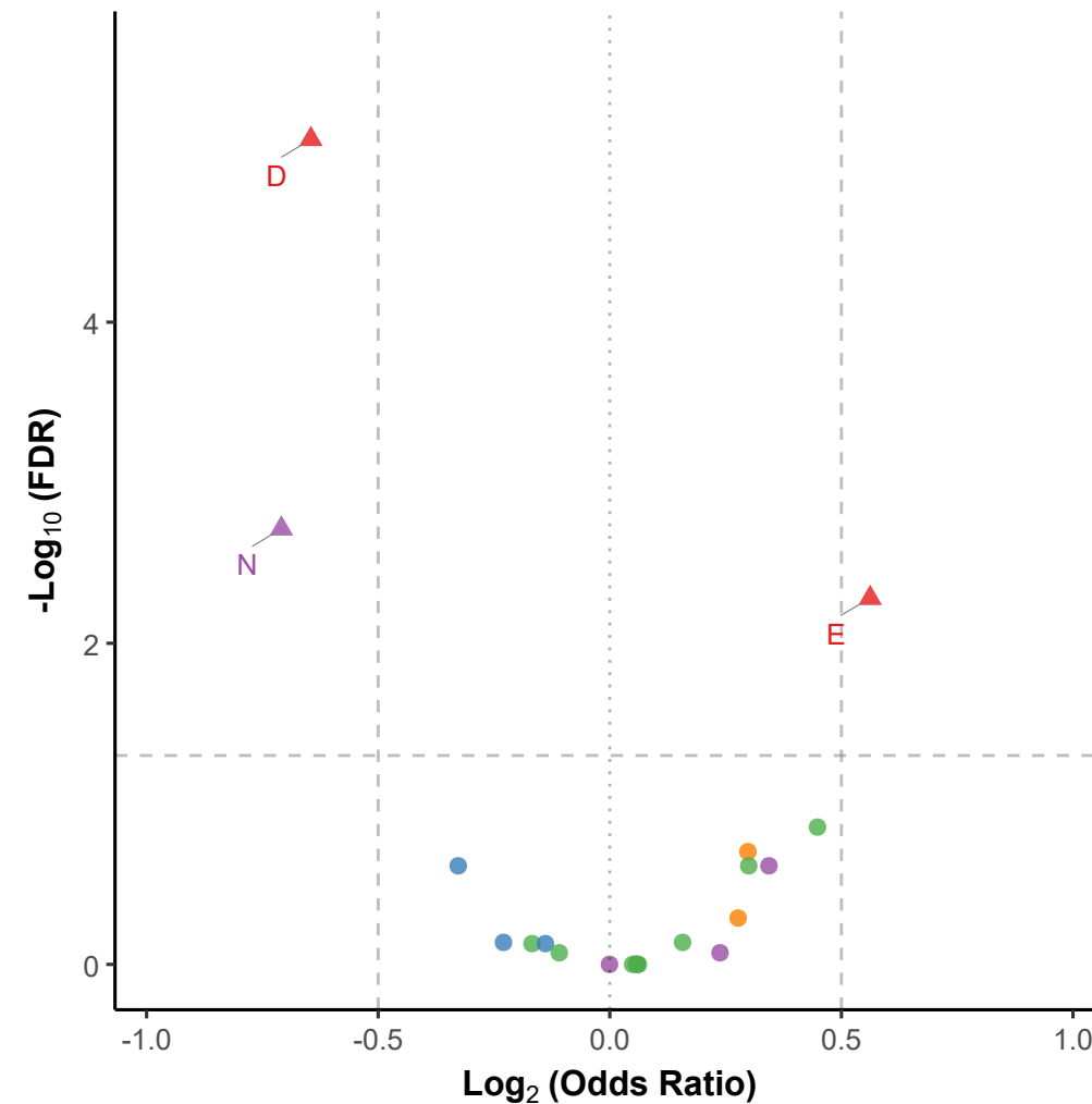
P-site
