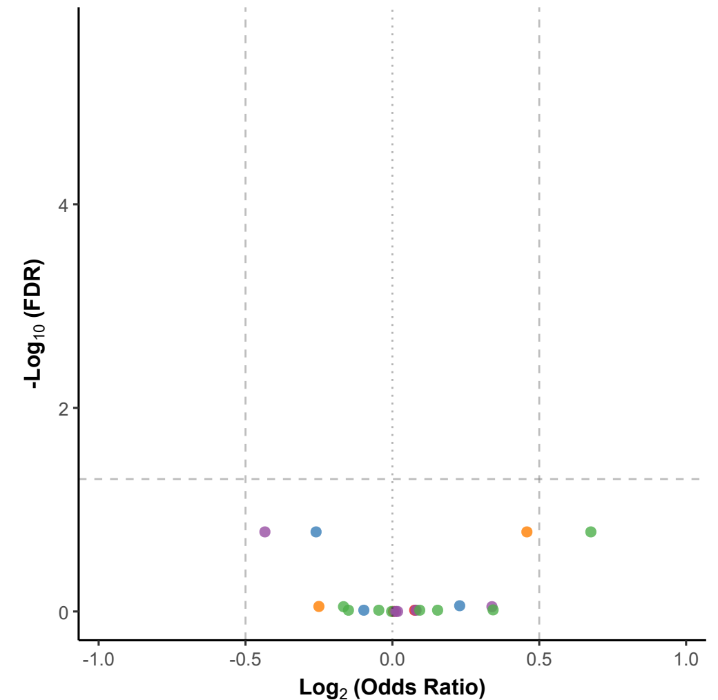
E-site
