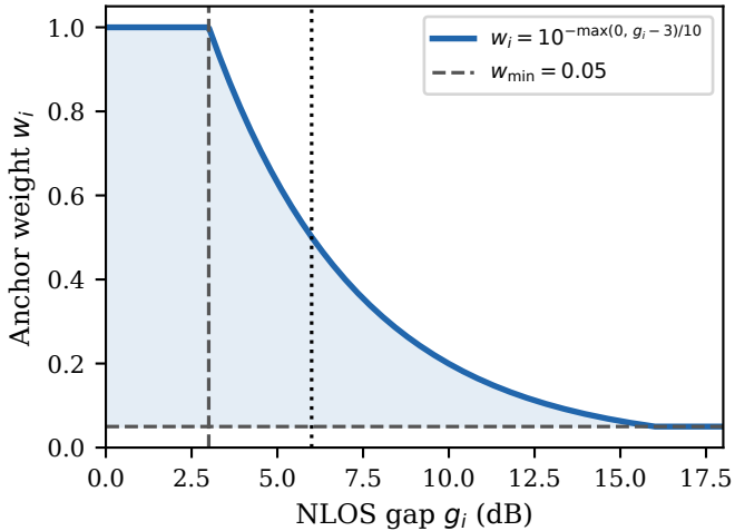
(b) LM weight as function of NLOS gap
