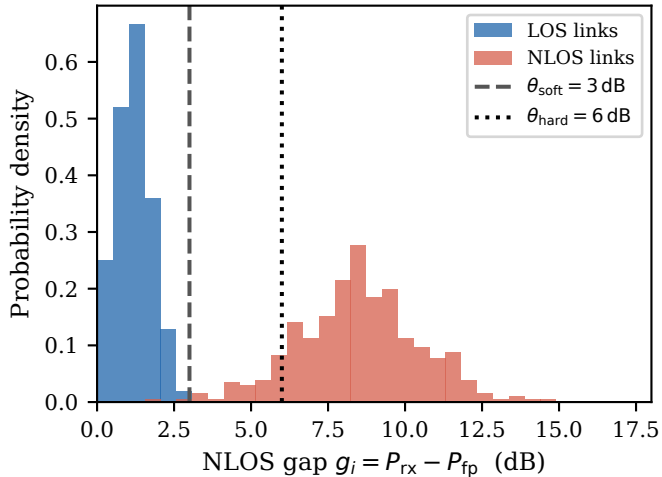
(a) LOS vs NLOS gap distribution (synthetic — replace with hardware data)
