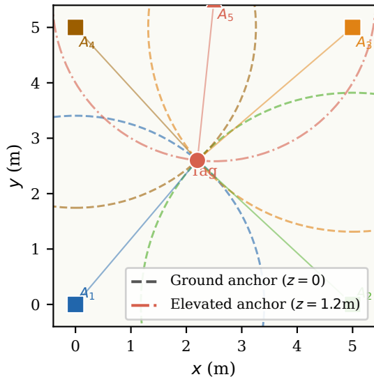
(b) 3D trilateration — 5 sphere projections
