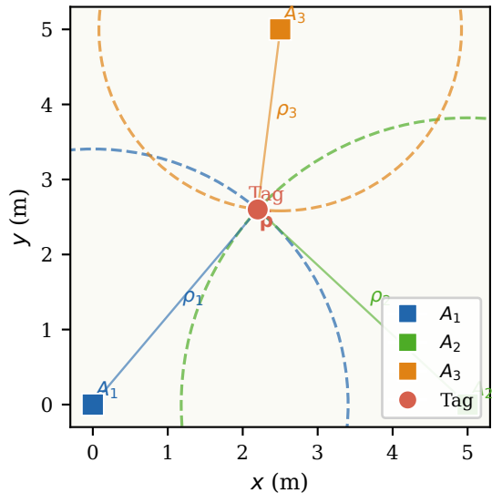
(a) 2D trilateration — 3 circle intersections
