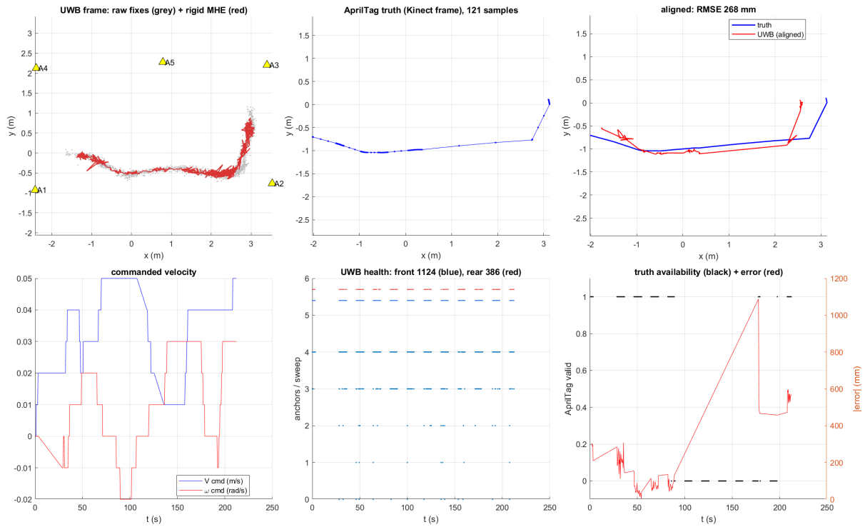
Figure 6: First driven run (212s). Top-left: raw fixes and the rigid-MHE track in the UWB frame. Top-middle: AprilTag truth. Top-right: the two overlaid after the fitted frame transform — the shapes agree. Bottom row: commanded velocities, UWB per-sweep health, truth availability with error over time.
