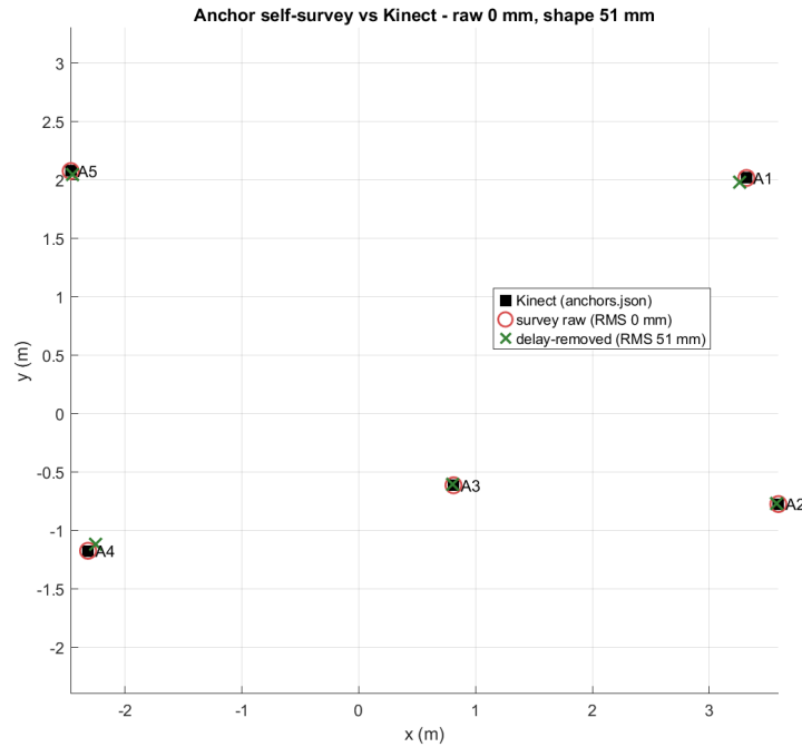
Figure 1: Self-survey vs the clicked-Kinect layout. Black squares: the camera’s anchors. Red circles: the survey shape (after a rotation/reflection alignment, since distances fix no absolute pose). Green crosses: the same after removing each anchor’s antenna-delay bias.
