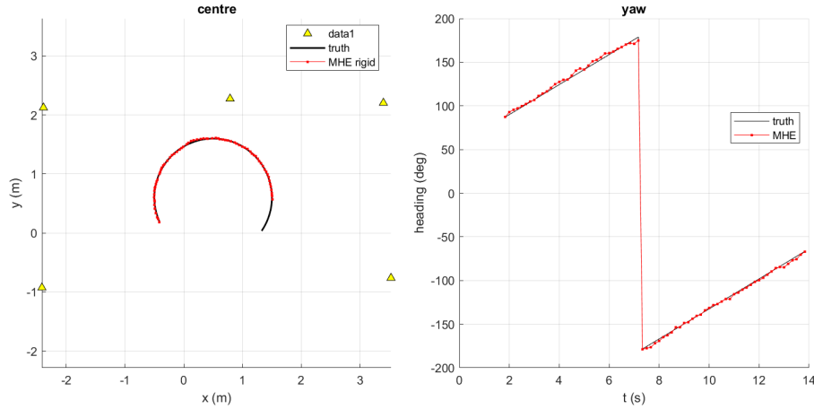
Figure 5: The synthetic validation: true arc (black) vs the rigid estimate (red), and true vs estimated heading. Zero guard trips.
