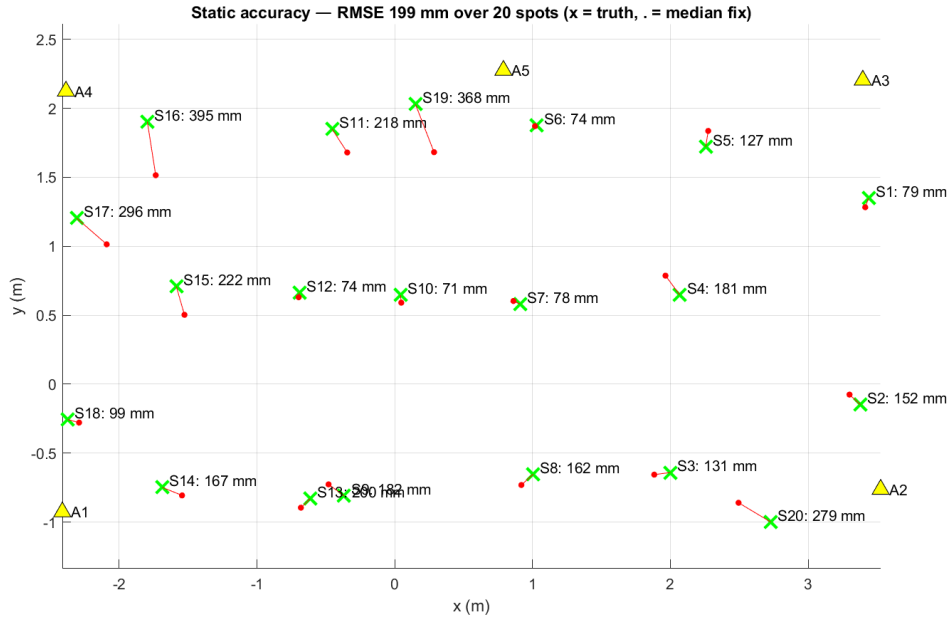
Figure 2: The static campaign: truth positions (green \times ), median solved positions (red dots), and per-spot error. The variation across the floor is the spatial error field that the power correction then largely removes.
