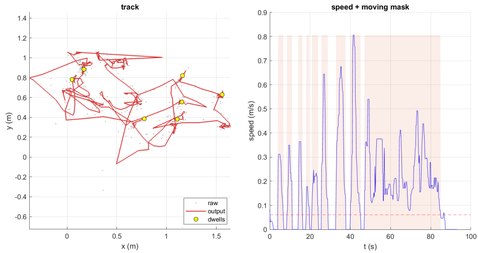
Figure 4: The hand-motion check that tuned the smoothing: raw fixes (grey), output track (red), detected dwells (yellow). Between-dwell displacements of the \sim 50 cm hand moves read 0.44–0.58 m — the poor man’s truth before the rover runs existed.
