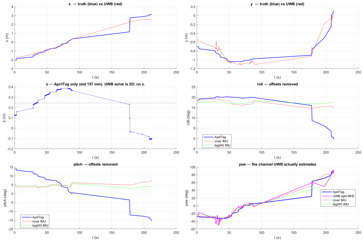
Figure 7: All six channels from the first run. Blue is the AprilTag; red/green are the two IMUs; magenta is the UWB rigid-MHE yaw. Note pitch and roll: the camera (blue) swings tens of degrees while the two independent IMUs agree with each other and stay flat — the camera is the outlier there.
