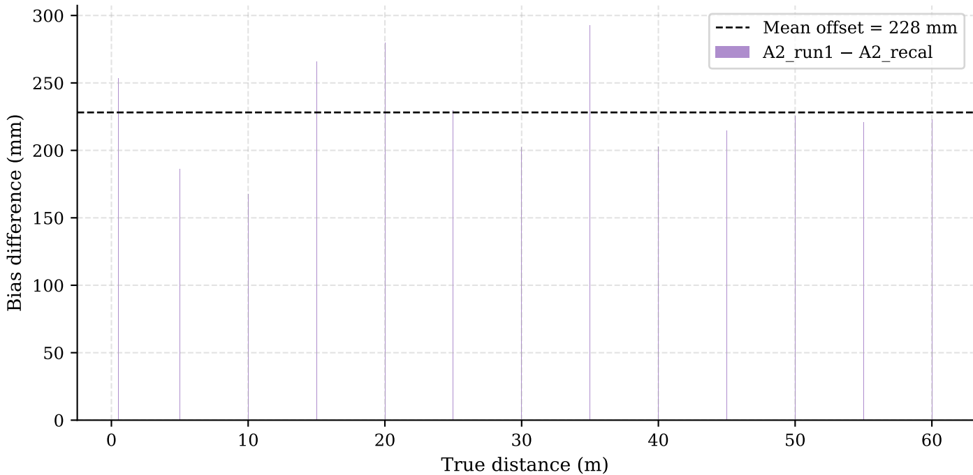
Bias Difference: Old Calibration – New Calibration (consistent ~228 mm shift = calibration error)
