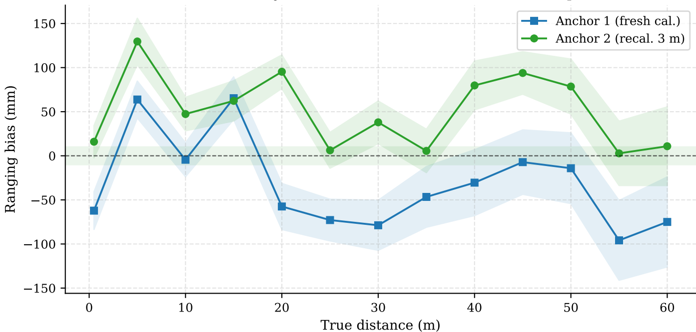
Anchor 1 – Anchor 2 Bias Difference RMS difference = 91 mm Range = [-153, 3] mm
