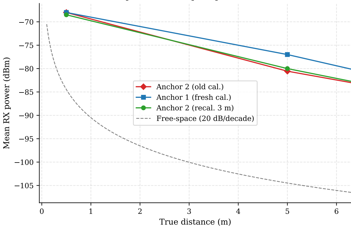
Received Power vs. Distance Compared to free-space path loss model
