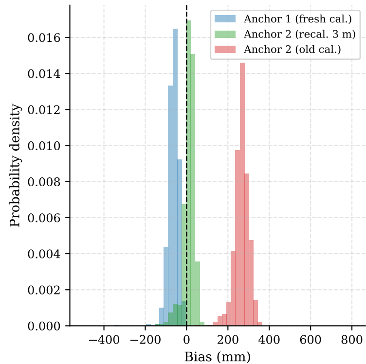
Near-field (5 cm) Distribution of bias
