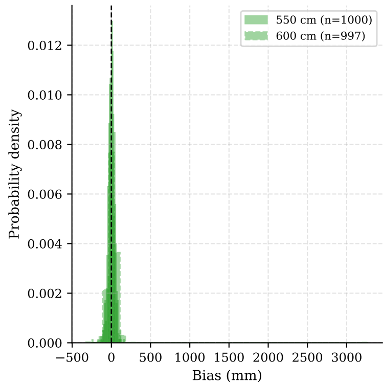
Long-range Distributions A2 recalibrated (550 & 600 cm)
