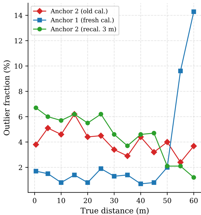
Outlier Rate vs. Distance (IQR 1.5 \times criterion)
