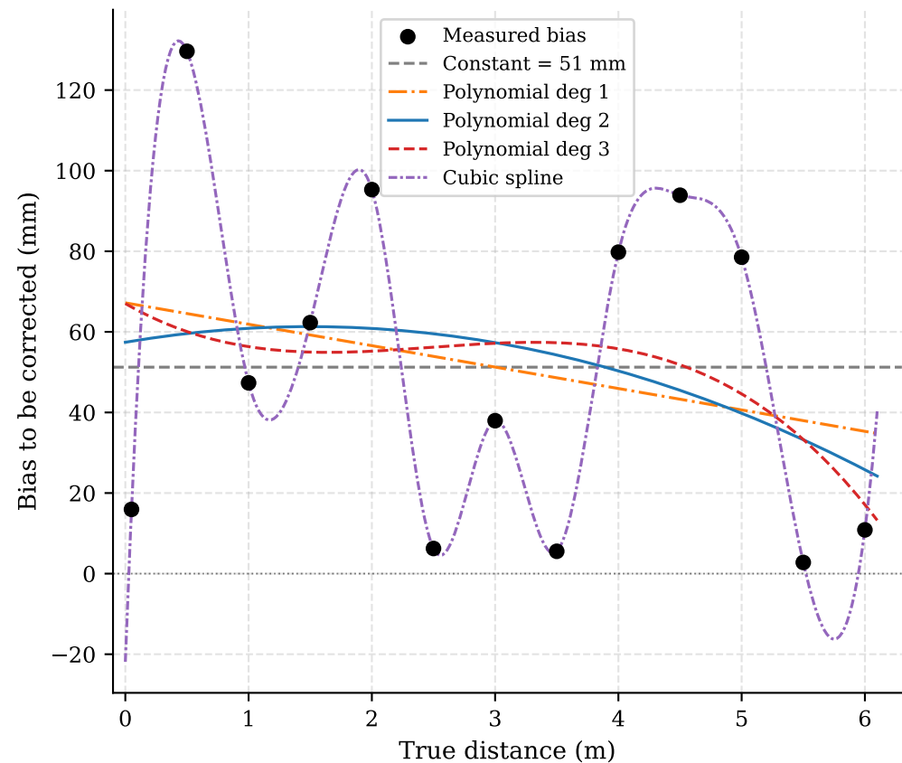
Correction Model Fits — A2 Recalibrated
