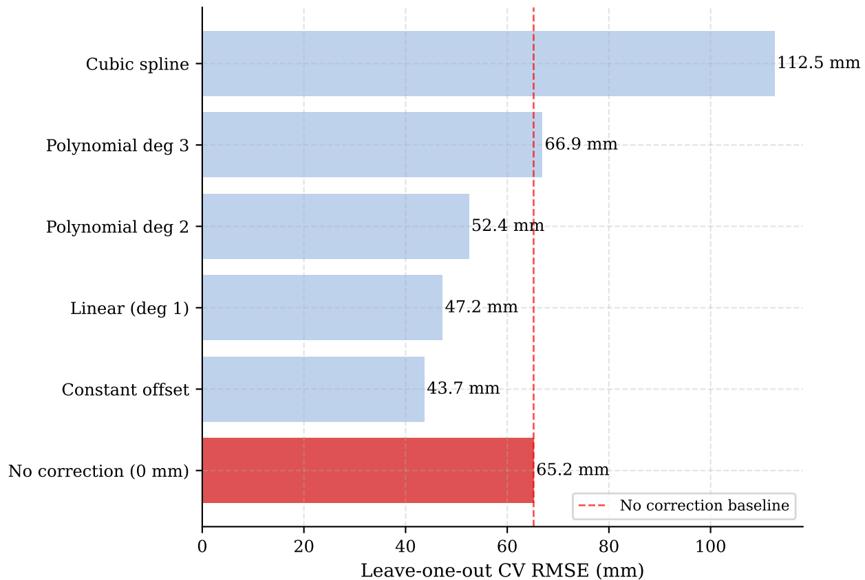
Cross-Validation RMSE by Correction Model (A2 recalibrated, all distances included)
