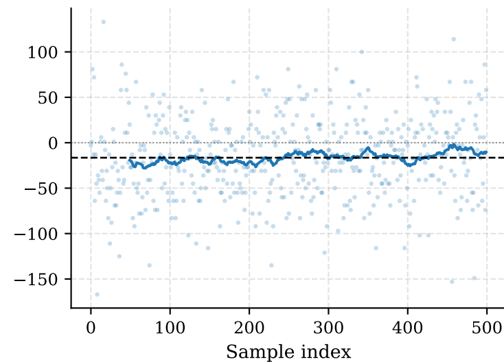
Anchor 2 (recal. 3 m) 500 cm, session 1
