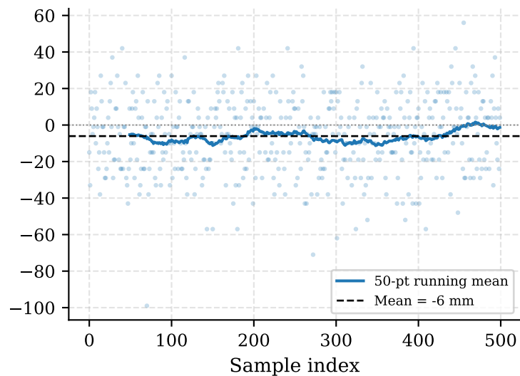
Anchor 2 (recal. 3 m) 100 cm, session 1
