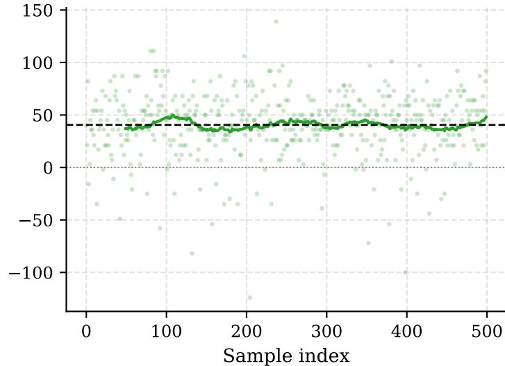
Anchor 2 (recal. 3 m) 300 cm, session 1
