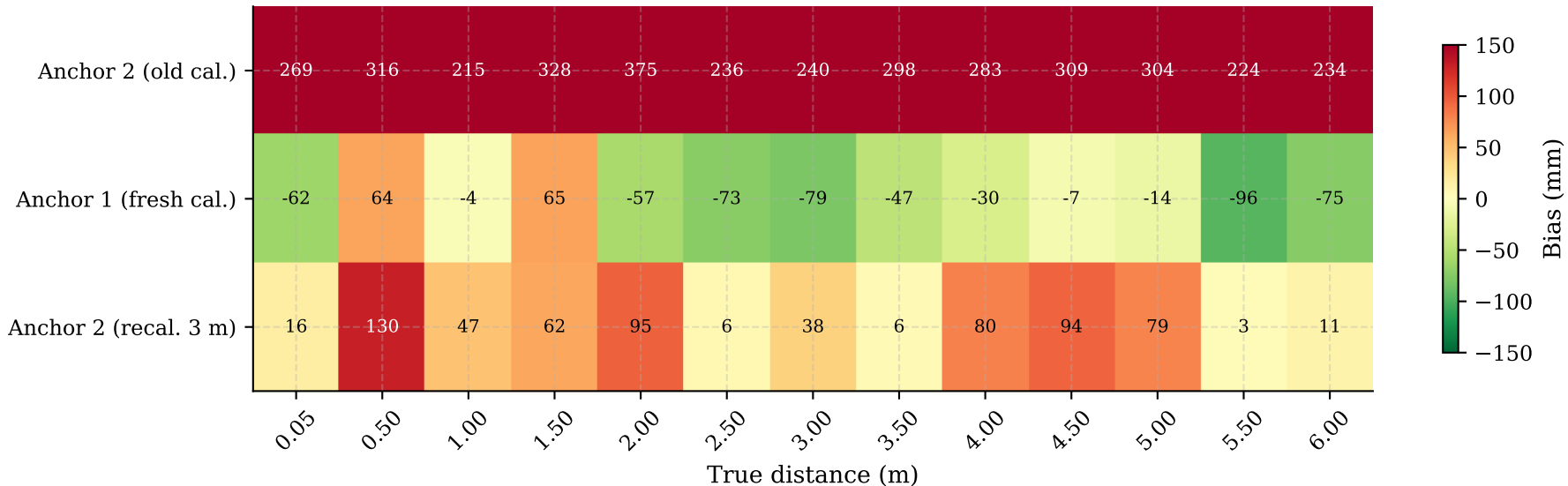
Bias Heatmap (mm): All Datasets × Distances (Green = near zero; Red = large positive/negative)
