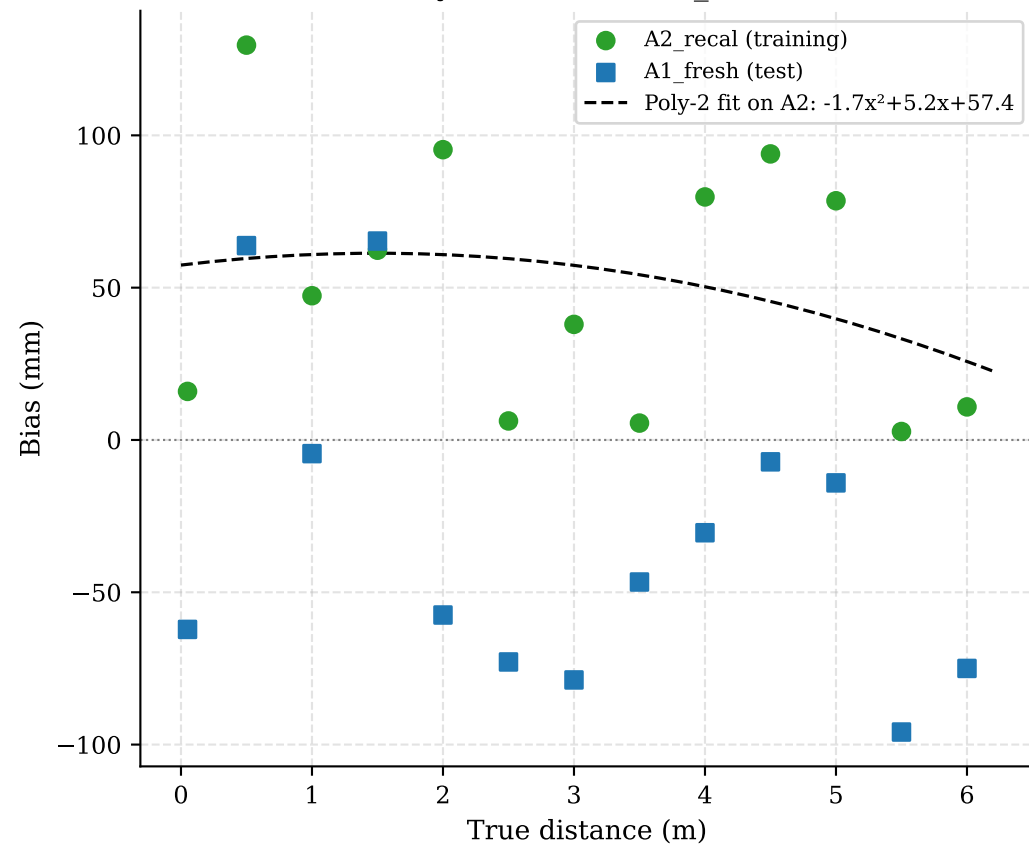
Cross-Archer Generalization Test Poly-2 trained on A2_recal
