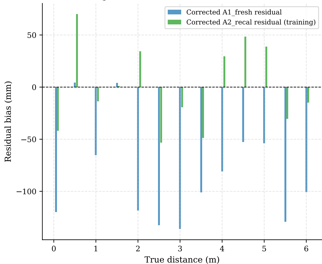
Residuals after Poly-2 Correction A2 (training) RMSE = 39 mm A1 (test) RMSE = 95 mm
