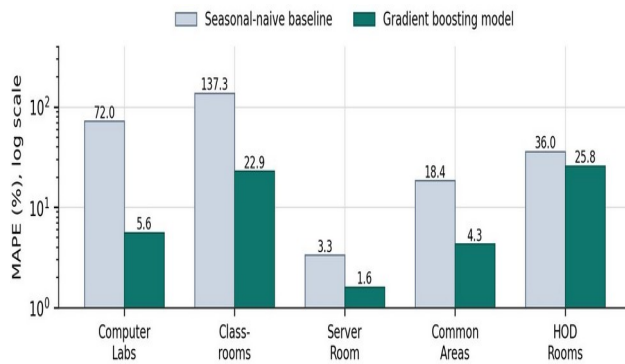
Fig. 2. Per-zone forecast MAPE against the recomputed seasonal-naive baseline, logarithmic scale, over non-anomalous test hours.
