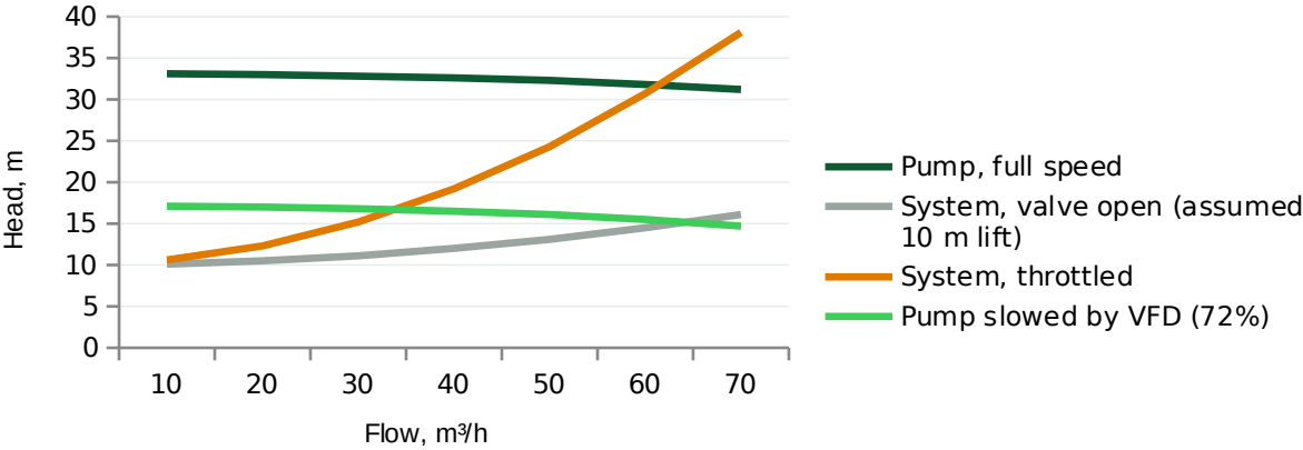
Grundfos NB 65-160/157 curves (fit to maker data)
