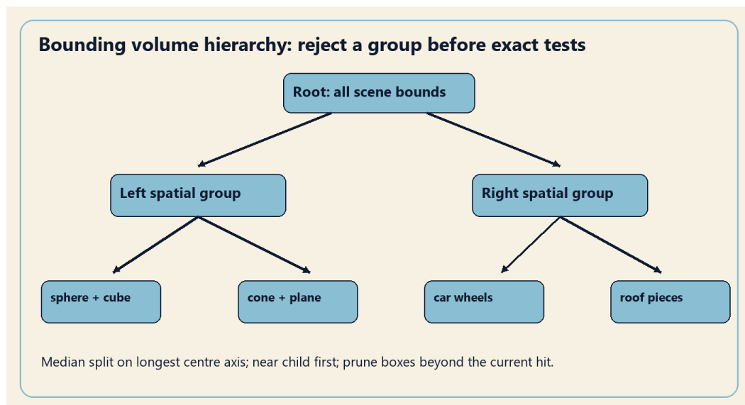
Figure 8: A spatial hierarchy rejects groups of distant objects before exact primitive intersection. The bounds must enclose the geometry after rotation, scale and shear.
