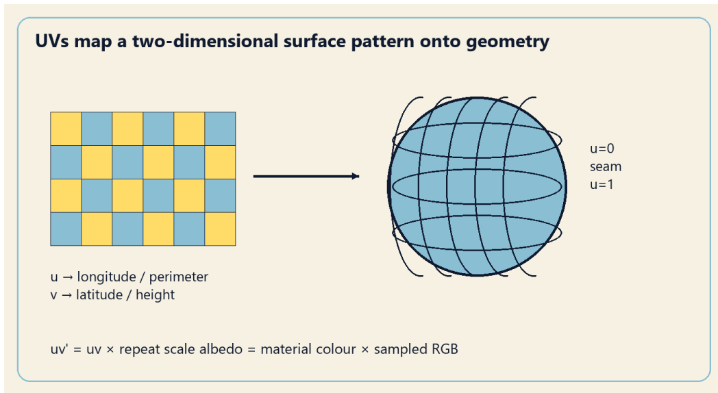
Figure 6: UV parameterisation and repeated surface detail. A duplicated seam separates u=0 from u=1 while keeping the same geometric position.
