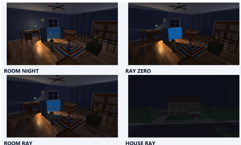
Figure 31: Raster room, zero-continuation primary view, two-continuation reflections and ray-traced exterior texture coverage.
