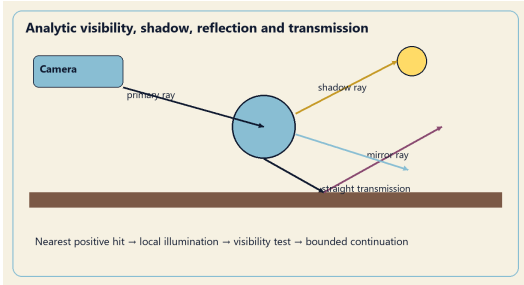
Figure 7: Primary, shadow, reflected and transmitted rays. A finite bounce budget limits tracing cost; the local surface model supplies each hit's colour.
