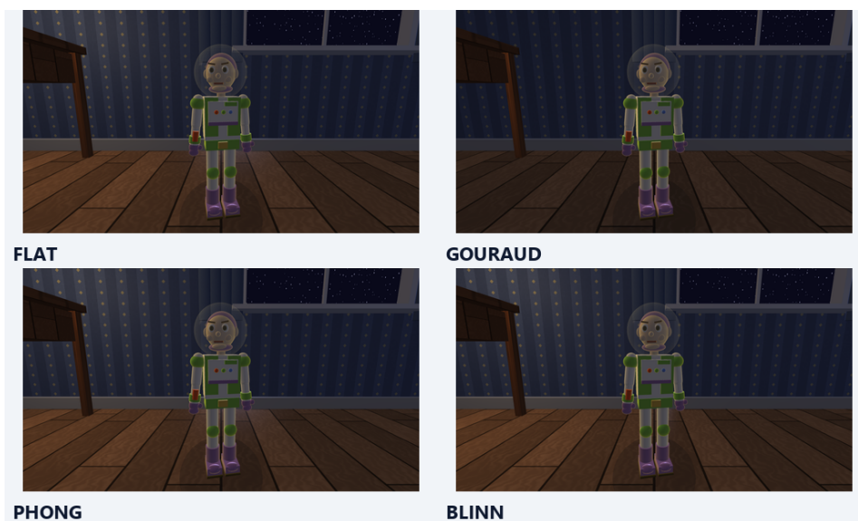
Figure 28: Matched Flat, Gouraud, Phong and Blinn-Phong views. The shading model changes while geometry, material and camera remain fixed.
