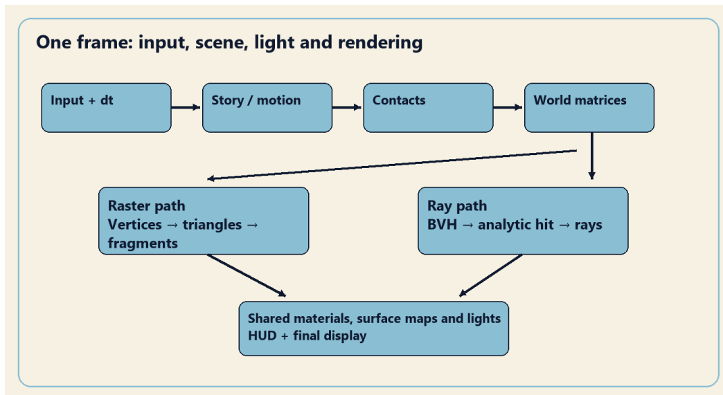
Figure 1: One frame from input to the displayed image. Both rendering paths consume the same scene transforms, materials and lights.
