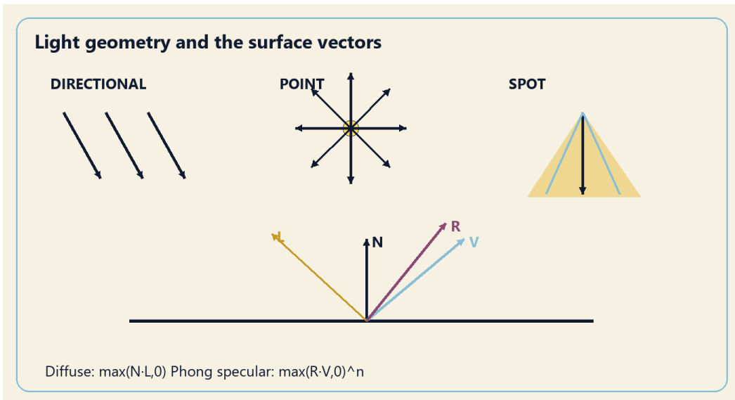
Figure 5: Directional, point and spot light geometry, followed by the normal, light, view and reflection vectors at a surface point.
