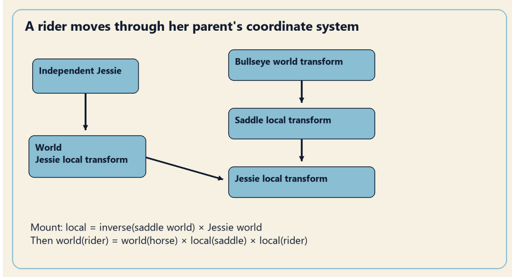
Figure 4: Jessie as an independent root and as a child of Bullseye’s saddle. The world-to-local conversion preserves placement before the seat transition.
