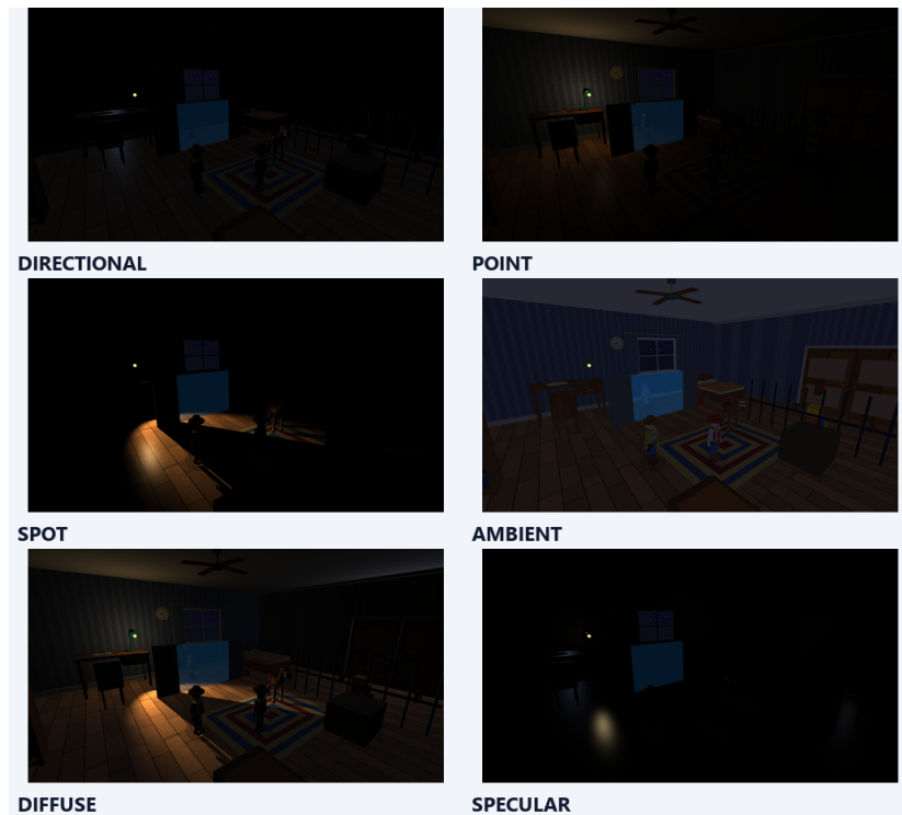
Figure 27: Isolated directional, point and spot sources (top rows), followed by ambient, diffuse and specular terms. All views are captured from the application.
