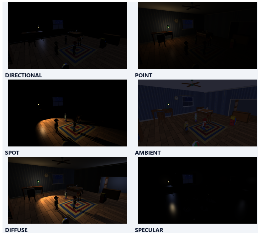
Figure 14: Isolated directional, point and spot sources (top rows), followed by ambient, diffuse and specular terms. All views are captured from the application.
