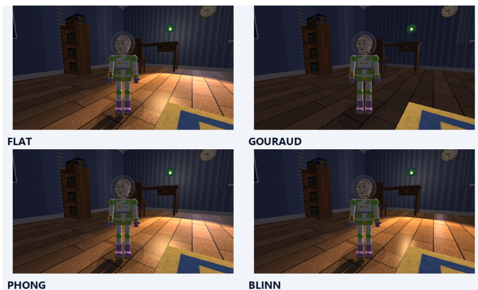
Figure 29: Matched Flat, Gouraud, Phong and Blinn-Phong views. The shading model changes while geometry, material and camera remain fixed.
