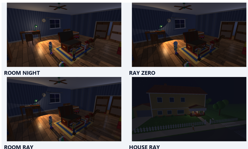
Figure 32: Raster room, zero-continuation primary view, two-continuation reflections and ray-traced exterior texture coverage.
