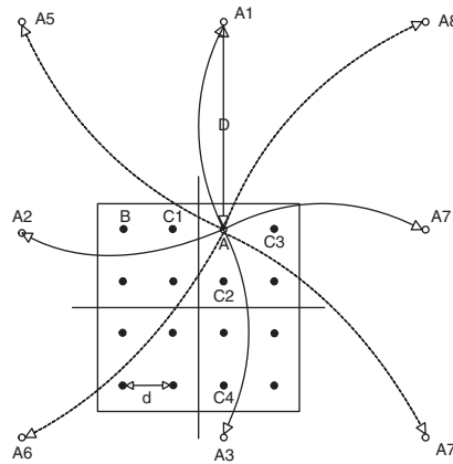
Figure 7.23 Expanded 16-QAM constellation for tone injection (TI) technique.
