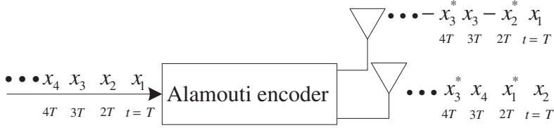
Figure 10.6 Alamouti encoder.
