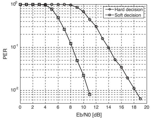
Figure 11.13 Packet error performance for SISO: hard decision vs. soft decision.
