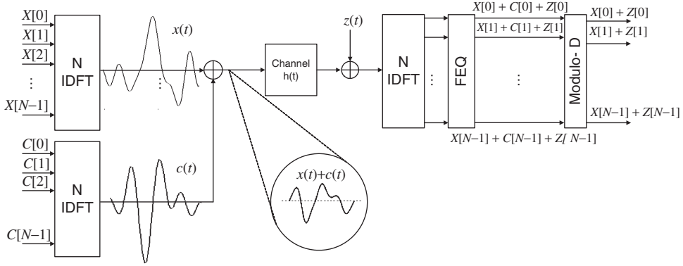
Figure 7.22 Block diagram of tone injection (TI) scheme.
