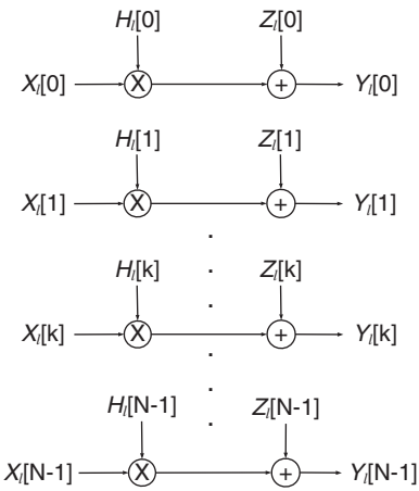
Figure 4.16 Frequency-domain equivalent model of OFDM system.
