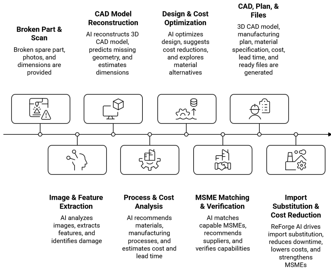
Fig.3 Workflow
