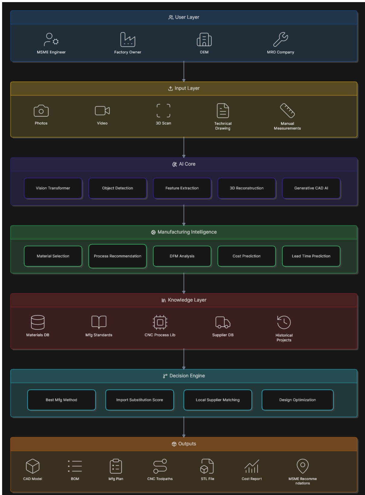
Fig.1 System Architecture
