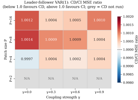
Figure 3: Leader-follower VAR(1): CD/CI test-MSE ratio across the (P, \gamma) grid, mean over seeds \{42, 123, 456, 789, 1011\} . Values above 1.0 favour CI. Coloured cells are the configurations where both modes were run ( P \in \{4, 8, 16\} ); the grey cells at P = 2 mark where CD exceeds T4 memory and was not run. Eleven of the twelve coloured cells favour CI and one ( P = 4, \gamma = 0.0 ) falls marginally below unity at 0.9997; the ratio stays within 0.15% of unity throughout.
