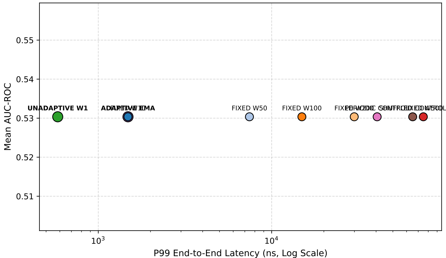
Figure 1: Latency-Accuracy Pareto Frontier Across Windowing Regimens
