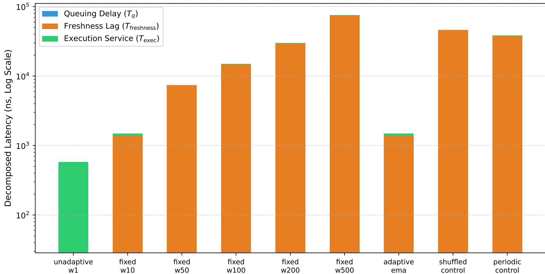
Figure 2: Decomposed Mean Latency Components ( T_q + T_{\text{freshness}} + T_{\text{exec}} )
