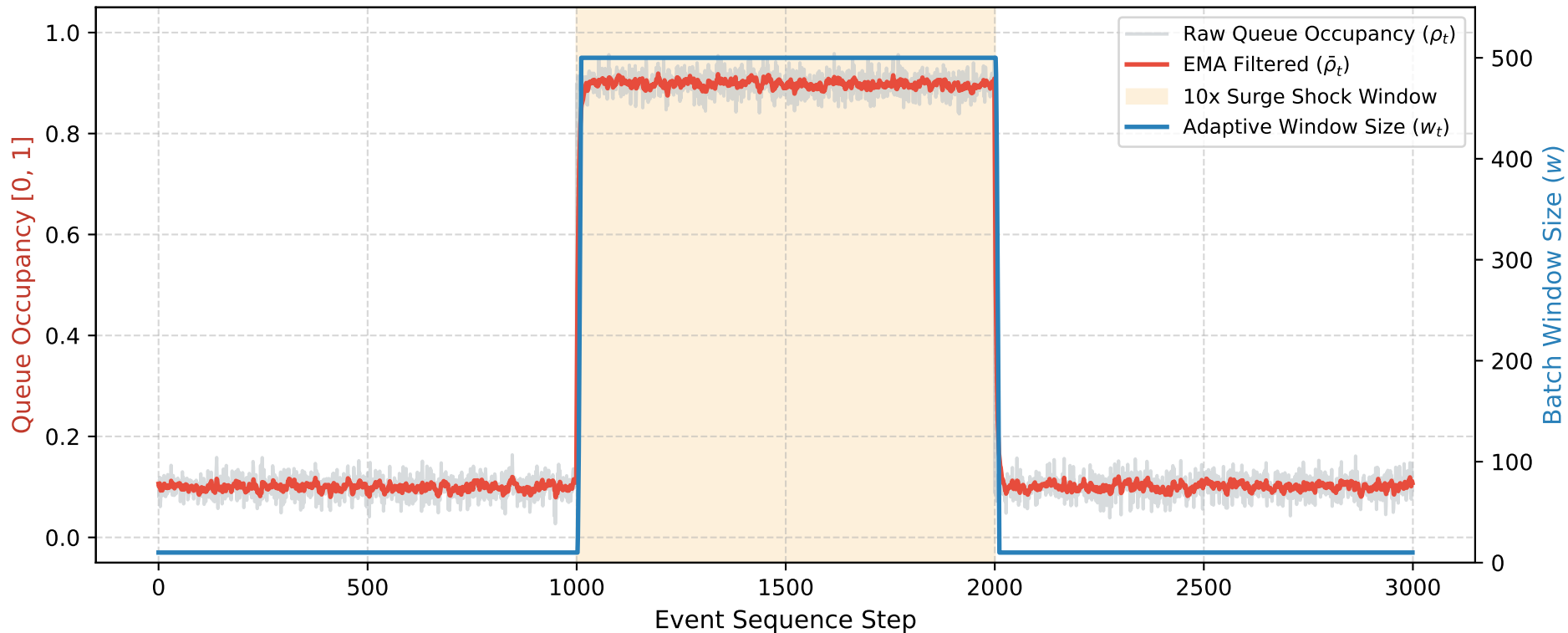
Figure 3: Transient Response and Damped Adaptation Under 10x Load Surge (MAR-X4)
