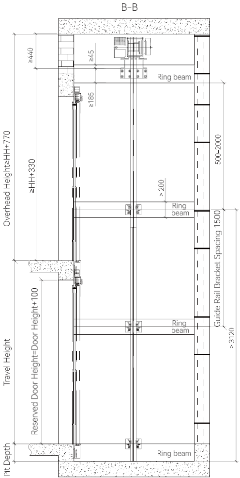
Shaft Section(Side Counterweight)
