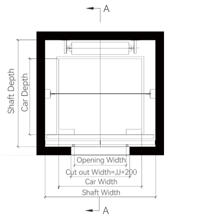
Shaft Plan(Rear Counterweight)
