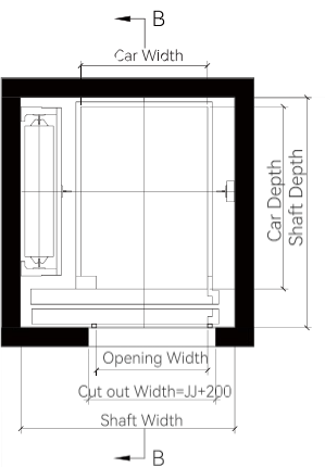
Shaft Plan(Side Counterweight)
