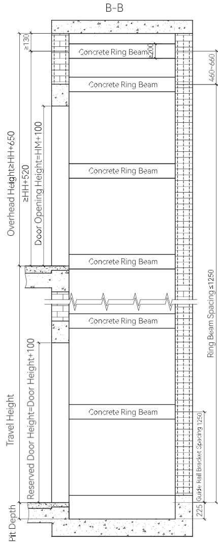
Shaft Section(Side Counterweight)
