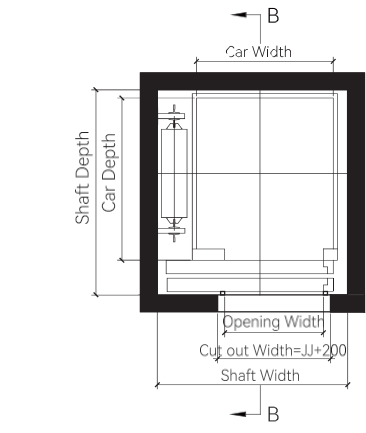
Shaft Plan(Side Counterweight)
