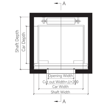
Shaft Plan(Rear Counterweight)
