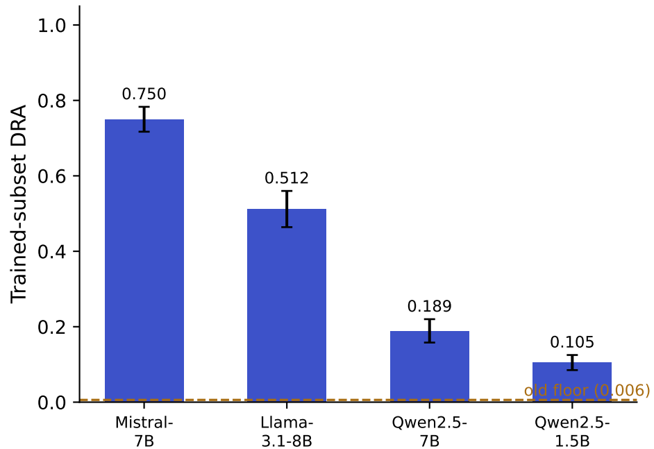
After: the localisation repair (mid-MLP + paraphrases + distillation, 5 seeds/model)
