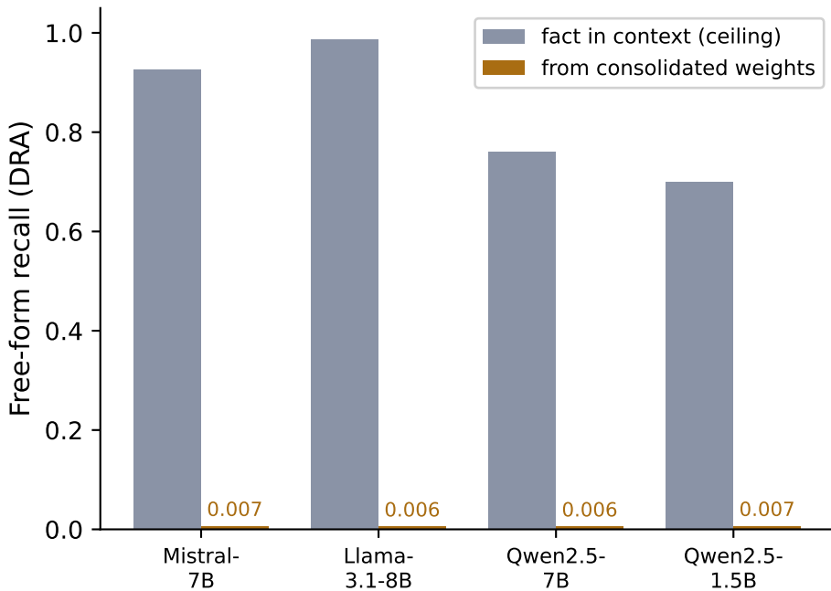
Before: recognition without recall (original placement, 5 seeds/model)
