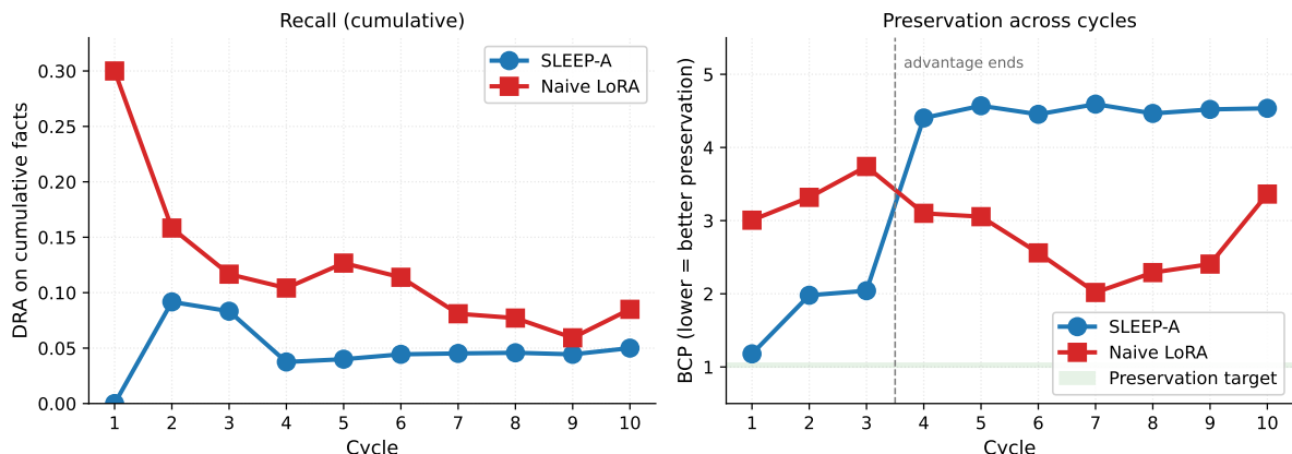
Figure 5: Ten-cycle continual learning on disjoint batches (Qwen2.5-7B, seed 0 shown; Table 6 reports all nine run-pairs). Left: cumulative DRA. Right: BCP with the crossover marked. SLEEP’s preservation advantage holds for three cycles, after which its BCP steps to a plateau while naive LoRA fluctuates.
