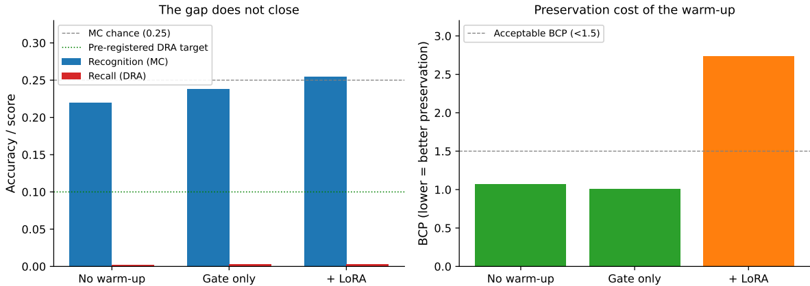
Figure 6: Warm-up extension results. Left: recognition (MC) and recall (DRA) under each condition; the pre-registered DRA target is marked. Recognition rises above chance while recall stays at floor. Right: the preservation cost, showing that the higher-capacity variant buys its small recognition gain with substantial base-capability degradation.
