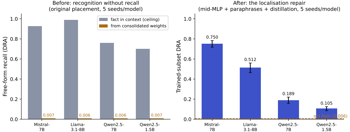
Figure 1: The paper in one figure. Left (the diagnosis): with the consolidation adapter placed by biological analogy (attention projections, top-third layers) and trained on single wordings, free-form recall from consolidated weights sits at \approx 0.006 on every model—while the same models answer from the same facts in context at up to 0.99. Right (the repair): relocating consolidation to mid-stack MLPs, training on paraphrase diversity, and distilling from an in-context teacher raises trained-subset recall to 17–125 \times the floor on every model (5 seeds each, error bars \pm SD), strongest on the family the recipe never saw during development. Llama-3.1-8B gains recall but exceeds our damage bar and is flagged not yet tuned (Section 7.11).
