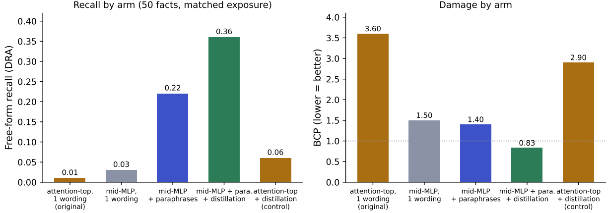
Figure 7: The localisation ladder (Qwen2.5-7B, 50 facts, matched exposure, clipping disabled; seed means—the mid-MLP single-wording arm’s BCP spans 1.2–1.8 across seeds and is drawn at its midpoint). Left: free-form recall by arm. Right: background damage. The same gradient budget, redirected from top-third attention to mid-stack MLPs, does less harm; paraphrase diversity and the distillation objective then convert the placement gain into recall— 60\times the original arm, at better-than-baseline preservation. The placement control (rightmost) shows the objective cannot rescue the wrong substrate.
