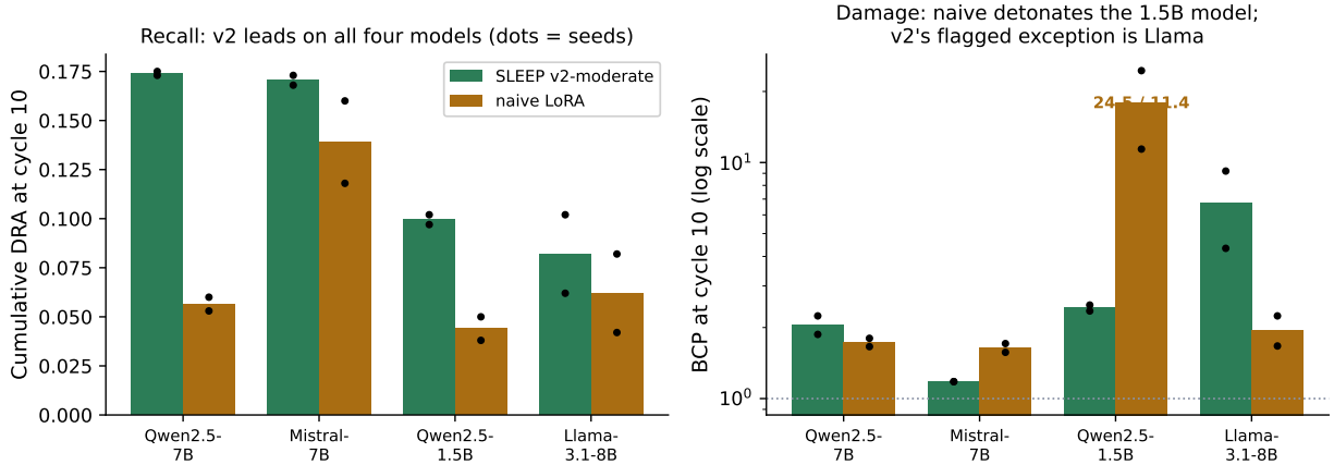
Figure 9: Ten-cycle endpoints across the matrix (bars = seed means, dots = individual seeds). Left: the repaired pipeline leads naive LoRA on cumulative recall on all four models. Right (log scale): damage—naive LoRA detonates the 1.5B model (BCP 24.5 and 11.4, seed-random size) while the constrained arm holds \approx 2.4 ; the constrained arm’s own flagged exception is Llama.
