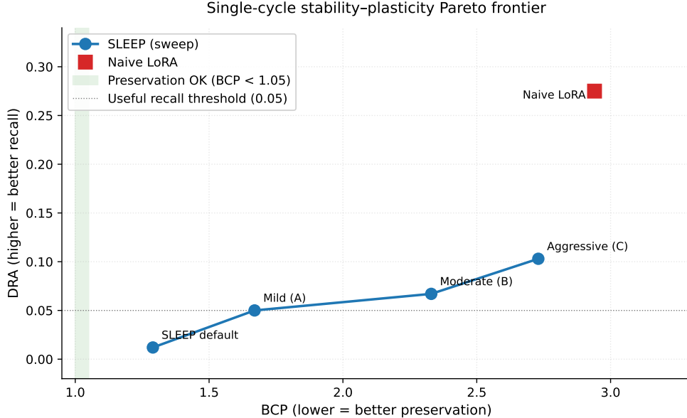
Figure 4: Single-cycle stability-plasticity Pareto frontier of the original architecture (attention-top placement, single-wording replay). The green band shows the preservation-acceptable region ( \text{BCP} < 1.05 ); the dotted line shows a useful-recall threshold ( \text{DRA} > 0.05 ). No setting on this frontier reaches the upper-left intersection—and Section 7.8 shows why: the frontier itself is an artefact of consolidating into the wrong substrate. The repaired pipeline of Section 7.10 reaches \text{DRA} = 0.189 at \text{BCP} = 0.88 on this model (five seeds), inside the region this curve suggested was unreachable.
