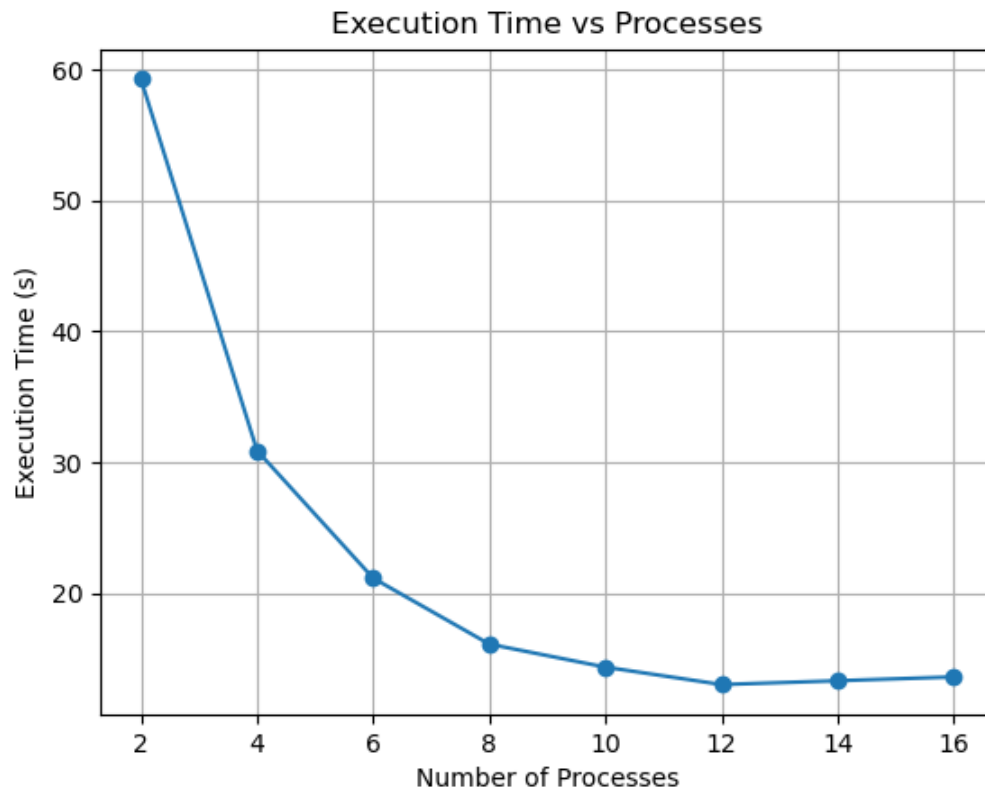
Figure 1: Performance across various runs
