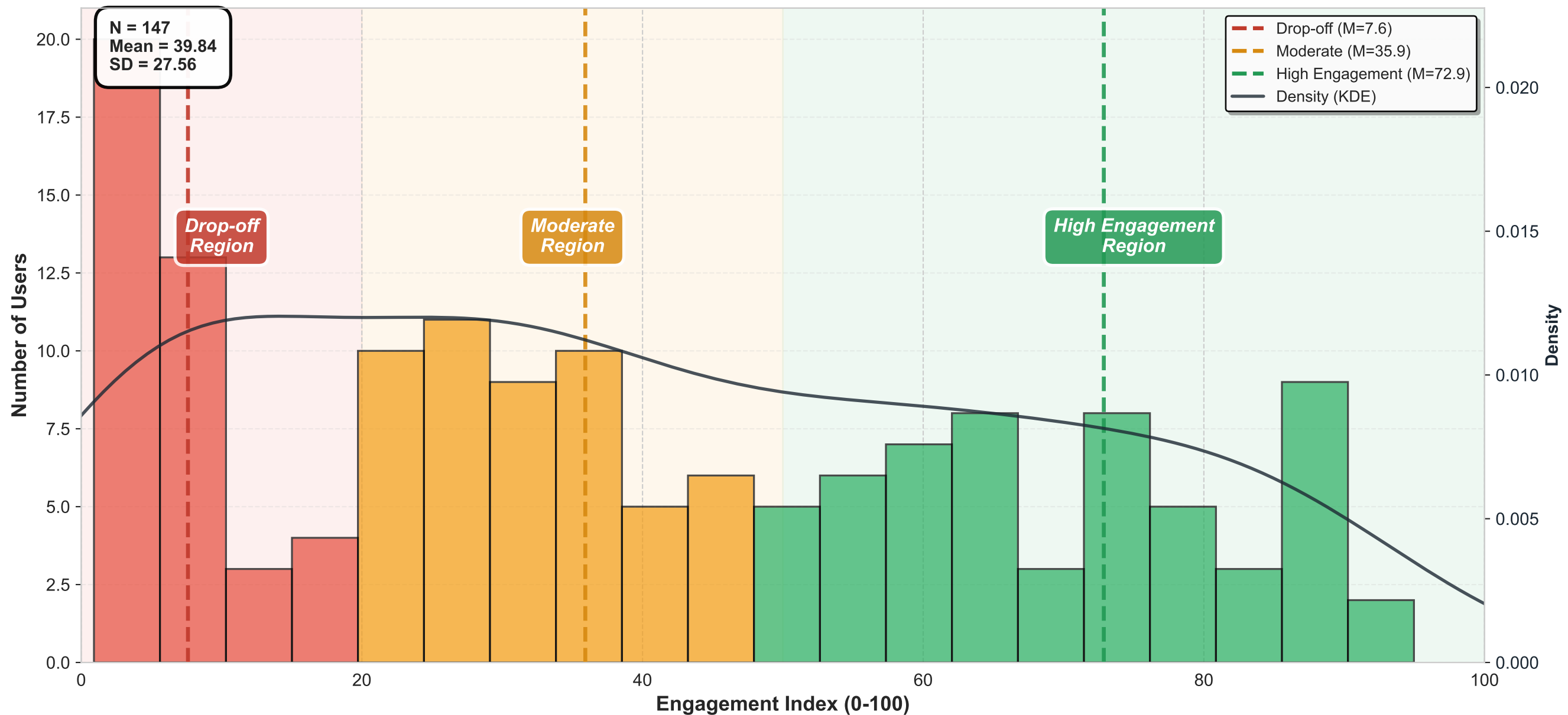
Engagement Index Distribution Across User Segments
