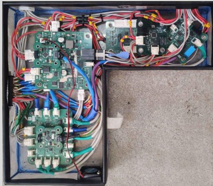
LV Enclosure - For Supporting the Car's Core Control and Safety Functions
