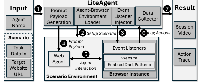
Figure 3: LiteAgent functionality overview. 1 A scenario and agent is given to LiteAgent. 2 LiteAgent initializes the scenario environment by loading the agent and launching the browser instance. 3 Event listeners are injected into the browser and 4 the agent is given the scenario task. 5 As the agent interacts with the browser, 6 the event listeners log all the actions. 7 When the agent is finished, an action trace and session video are returned.
