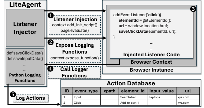
Figure 4: LiteAgent’s event listener injection and action logging pipeline. ① LiteAgent injects JavaScript event listeners into the browser’s context and ② exposes Python logging functions to these listeners. ③ When an event listener is triggered by an action, ④ the Python logging function is called and ⑤ logs the action into an action database.
