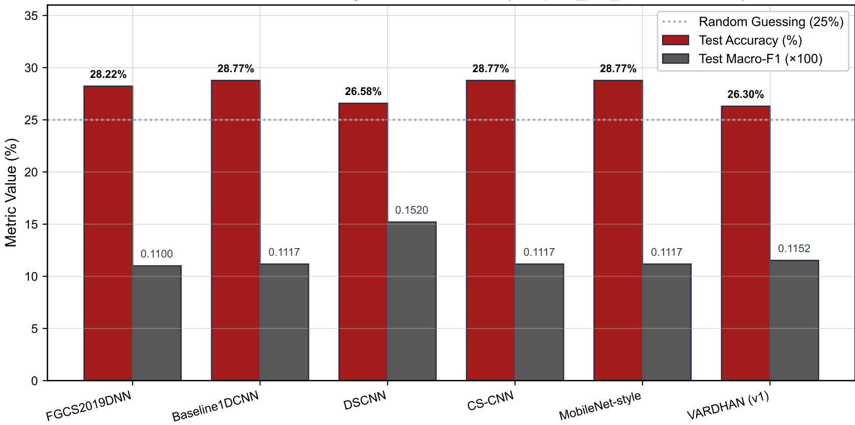
Historical Strict Recording-Level Benchmark (samples_per_file = 5, Seed 42)
