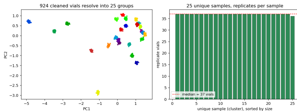
Figure 9: Answer to part (h). Left: the 924 cleaned vials, coloured by cluster, separate into 25 distinct groups in the leading covariance-score plane (some groups overlap in this 2-D view but are resolved in the full four-dimensional projection). Right: the replicate count per group is nearly constant at \sim 37 vials ( 24 \times 37 + 36 = 924 ), the signature of a designed taste test with 25 unique samples.
