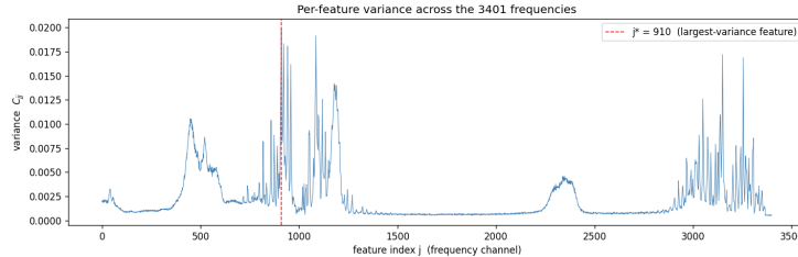
Figure 4: Per-feature variance C_{jj} across the 3401 frequencies, with the maximum at j^\star = 910 (dashed). Variance lives in a handful of molecular bands, not the baseline.
