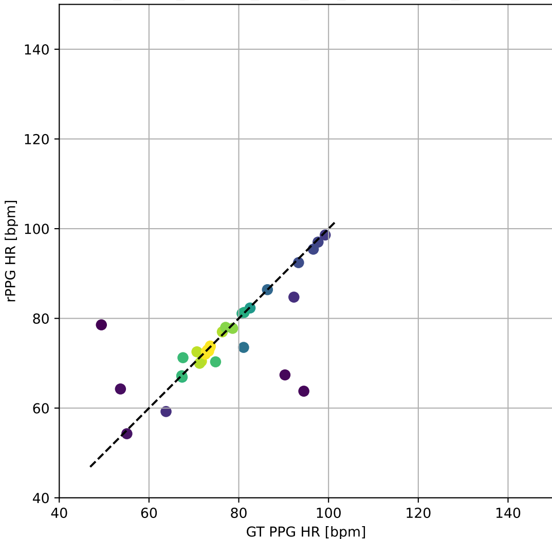
MMPD_5FOLD_physnet_fold1_FFT_BlandAltman_ScatterPlot
