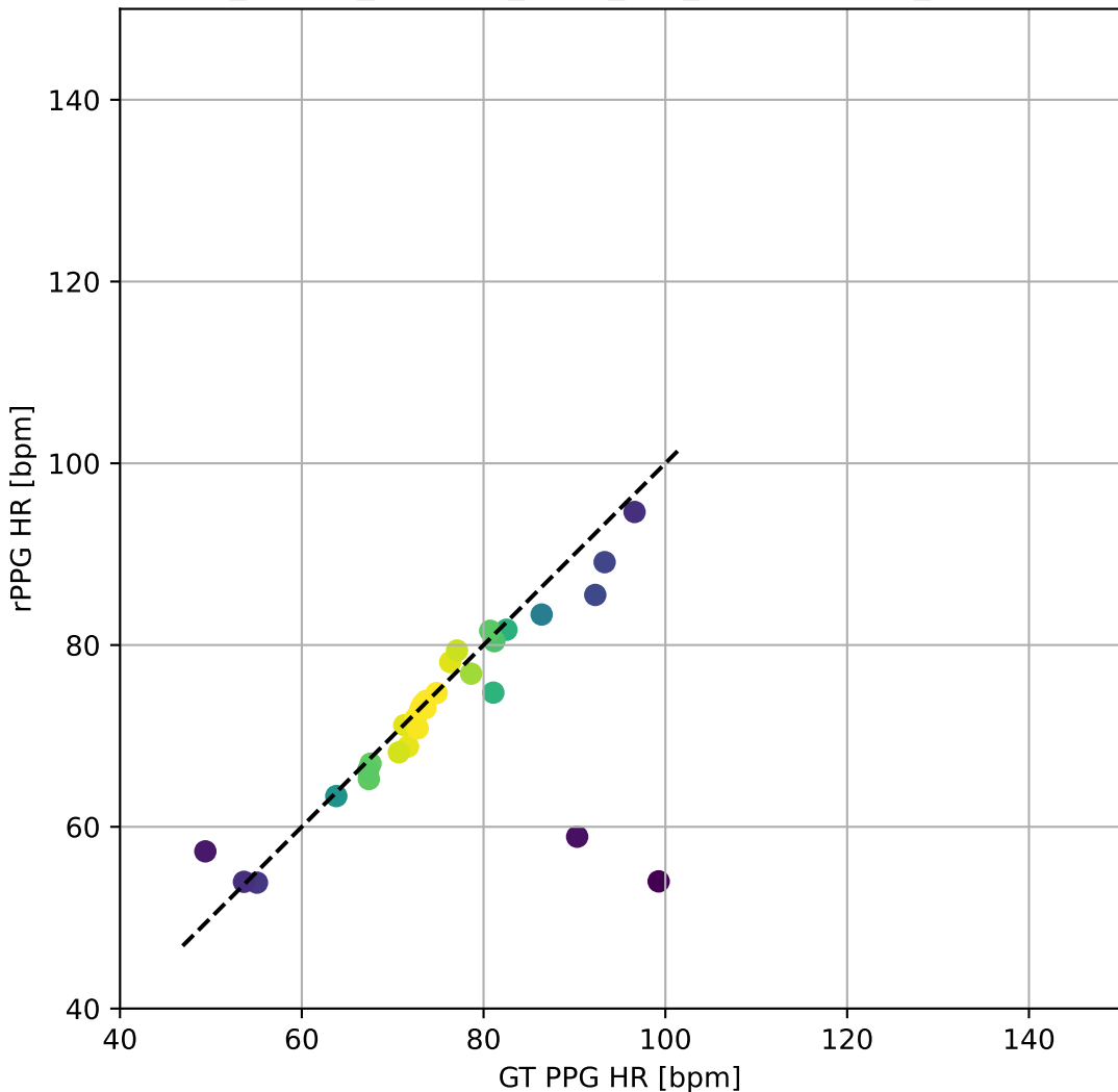
MMPD_5FOLD_physnet_fold2_FFT_BlandAltman_ScatterPlot
