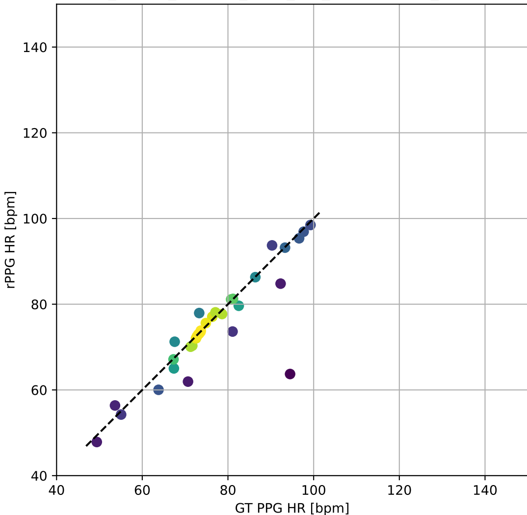
MMPD_5FOLD_physnet_fold4_FFT_BlandAltman_ScatterPlot
