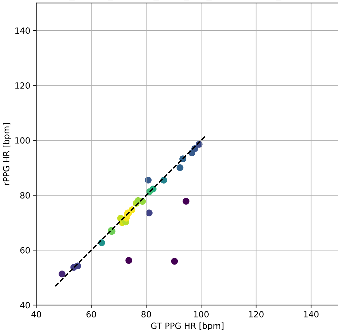
MMPD_5FOLD_physnet_fold5_FFT_BlandAltman_ScatterPlot
